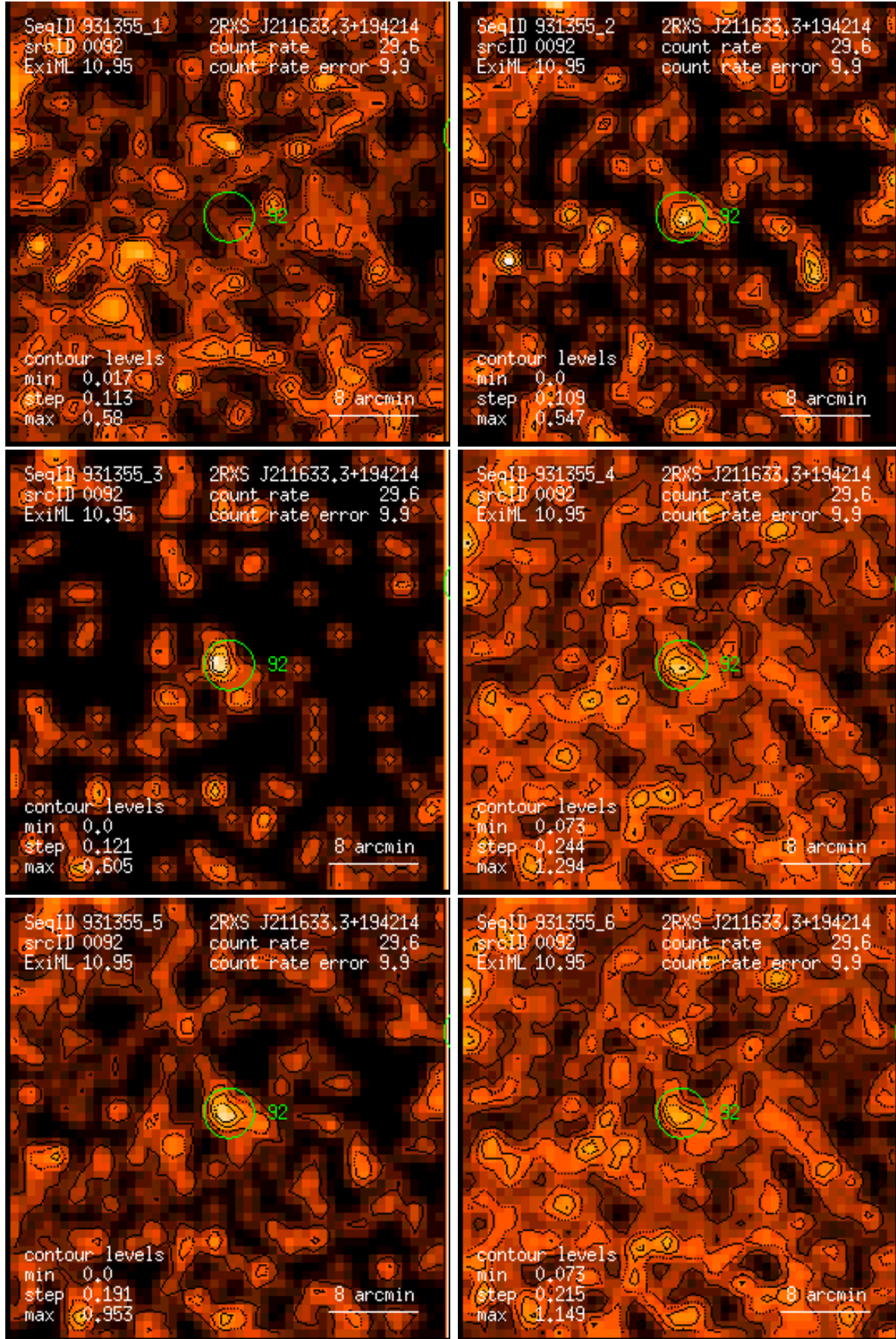
Figure 92: RASS 931355: detection 0092: band rate images, Gaussian filter: (1) PSPC channels 11 – 41, (2) 52 – 90, (3) 91 – 201, (4) 11 – 235, (5) 52 – 201, (6) 11 – 201. Broad band rates in counts/ks. Band rate contour levels in counts/ks/arcmin 2 .
