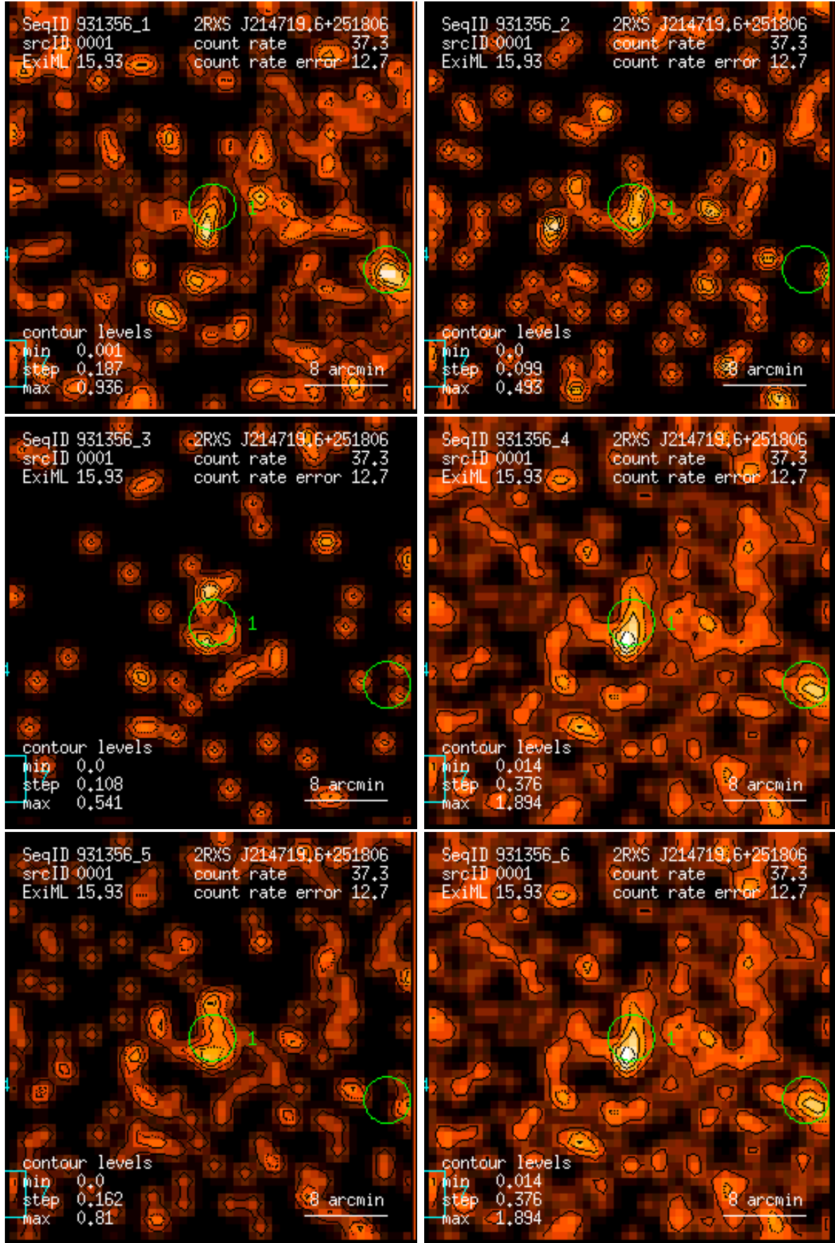
Figure 1: RASS 931356: detection 0001: band rate images, Gaussian filter: (1) PSPC channels 11 – 41, (2) 52 – 90, (3) 91 – 201, (4) 11 – 235, (5) 52 – 201, (6) 11 – 201. Broad band rates in counts/ks. Band rate contour levels in counts/ks/arcmin 2 .
