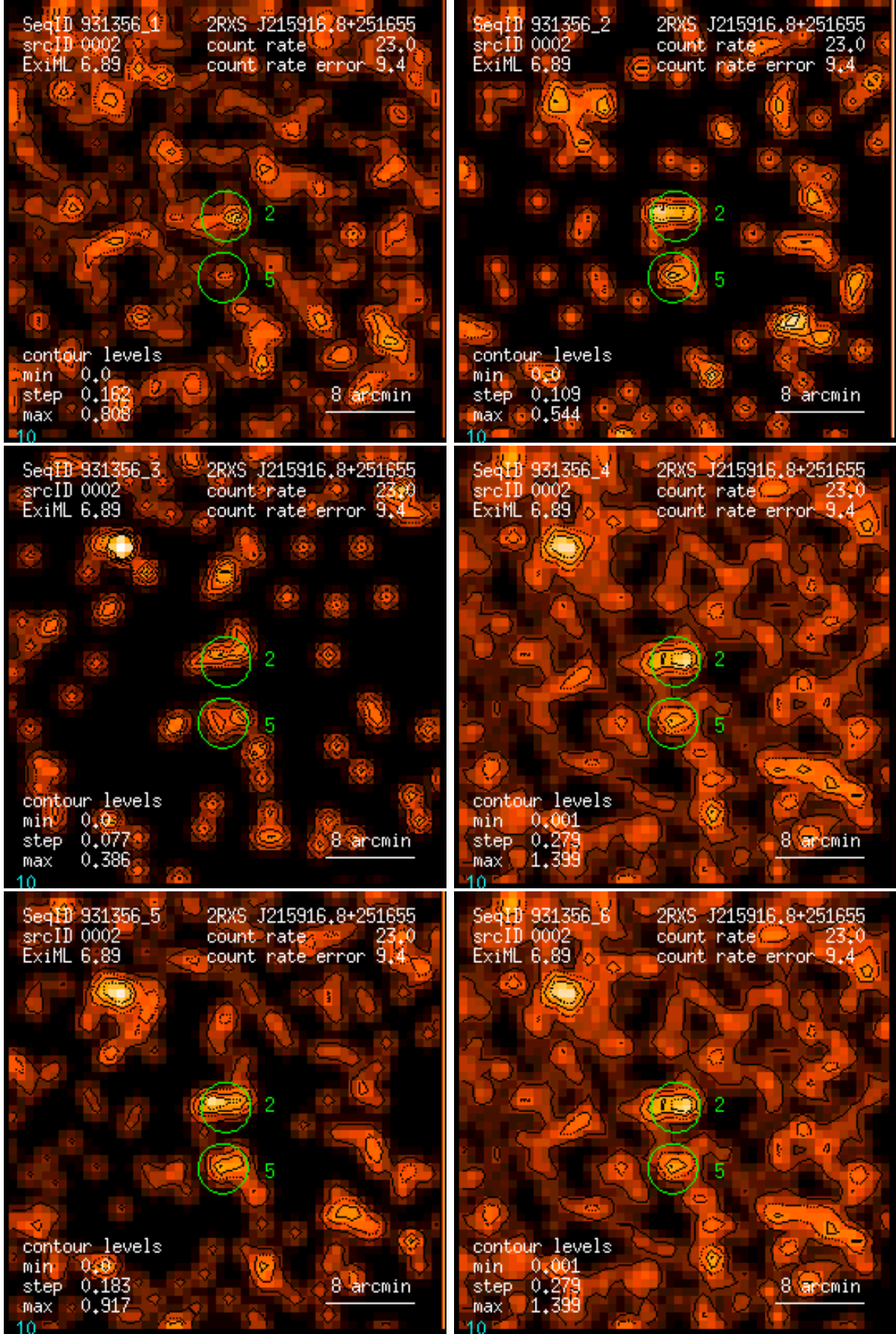
Figure 2: RASS 931356: detection 0002: band rate images, Gaussian filter: (1) PSPC channels 11 – 41, (2) 52 – 90, (3) 91 – 201, (4) 11 – 235, (5) 52 – 201, (6) 11 – 201. Broad band rates in counts/ks. Band rate contour levels in counts/ks/arcmin 2 .
