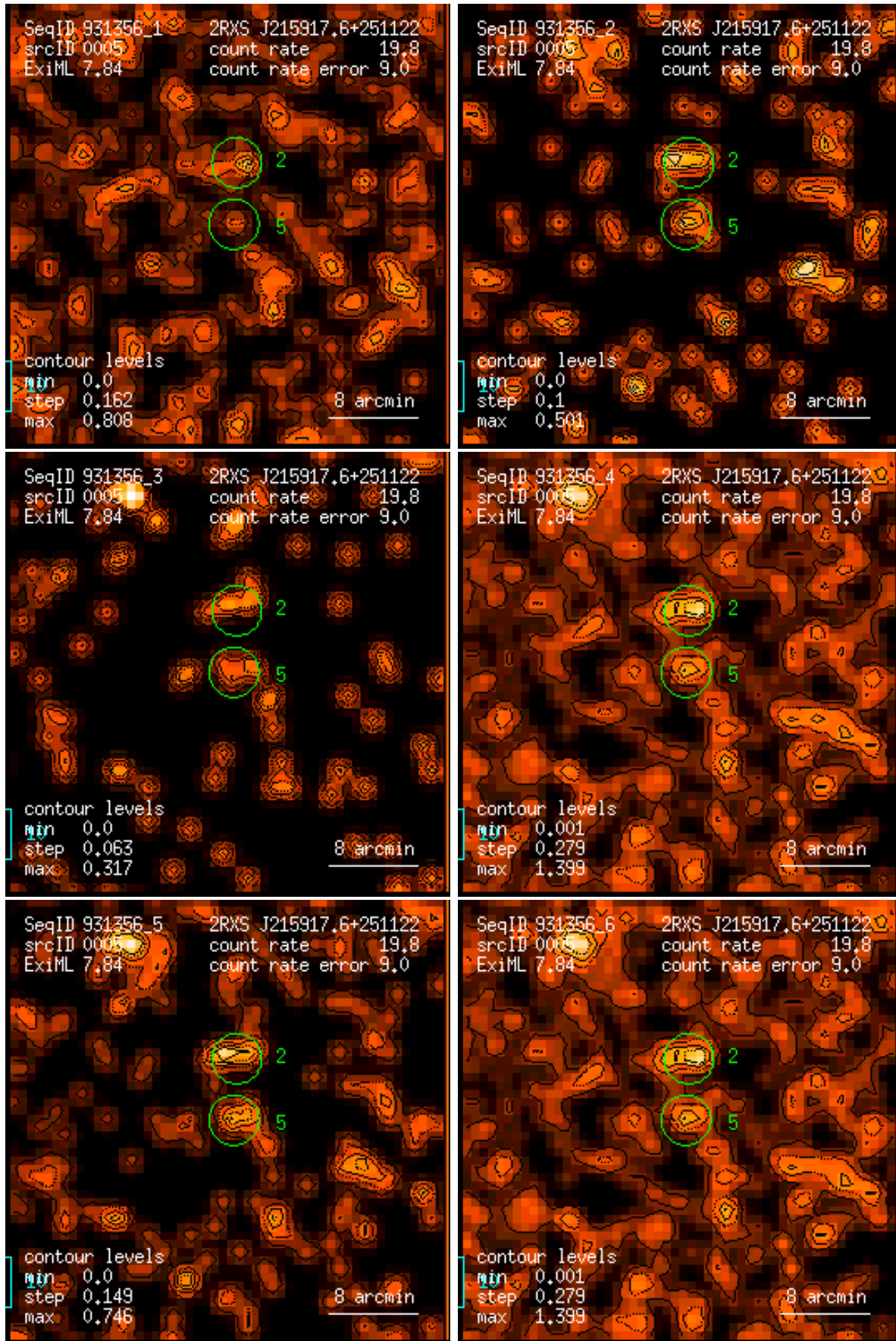
Figure 5: RASS 931356: detection 0005: band rate images, Gaussian filter: (1) PSPC channels 11 – 41, (2) 52 – 90, (3) 91 – 201, (4) 11 – 235, (5) 52 – 201, (6) 11 – 201. Broad band rates in counts/ks. Band rate contour levels in counts/ks/arcmin 2 .
