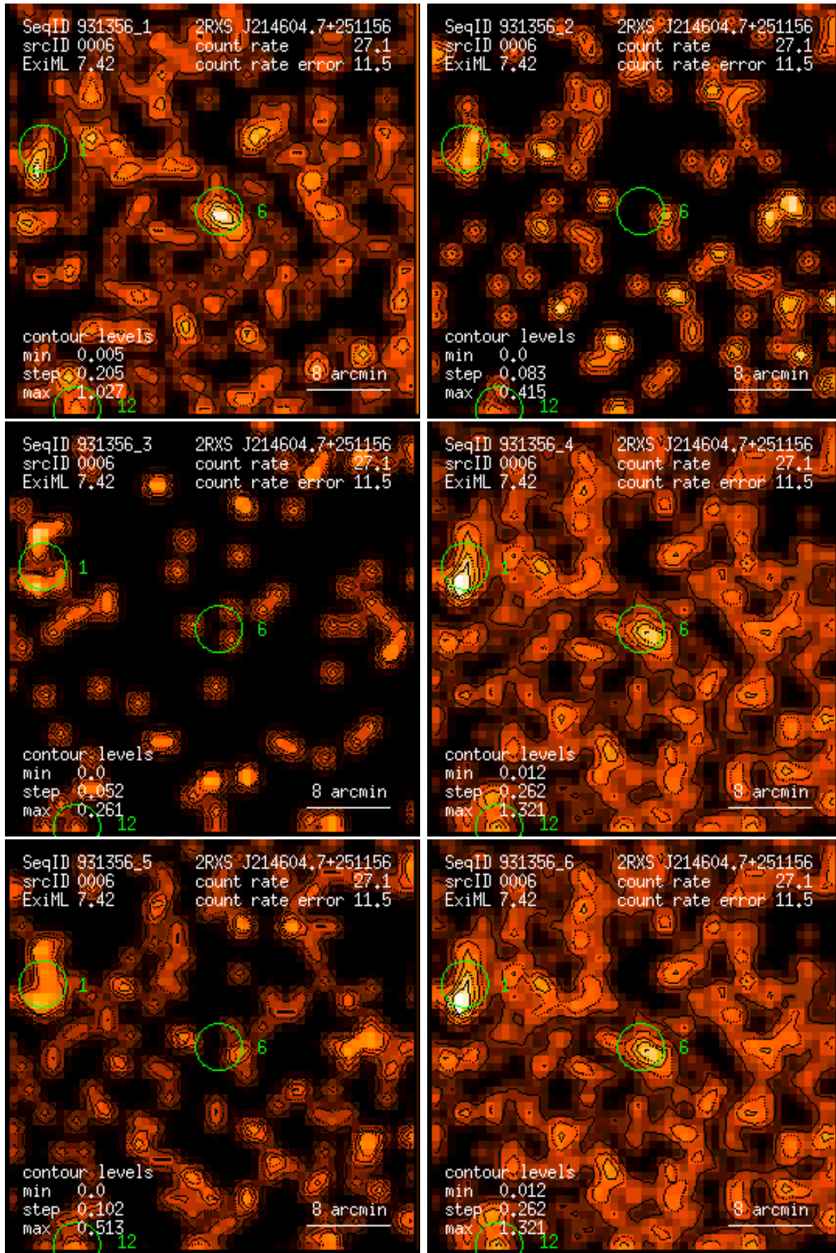
Figure 6: RASS 931356: detection 0006: band rate images, Gaussian filter: (1) PSPC channels 11 – 41, (2) 52 – 90, (3) 91 – 201, (4) 11 – 235, (5) 52 – 201, (6) 11 – 201. Broad band rates in counts/ks. Band rate contour levels in counts/ks/arcmin 2 .
