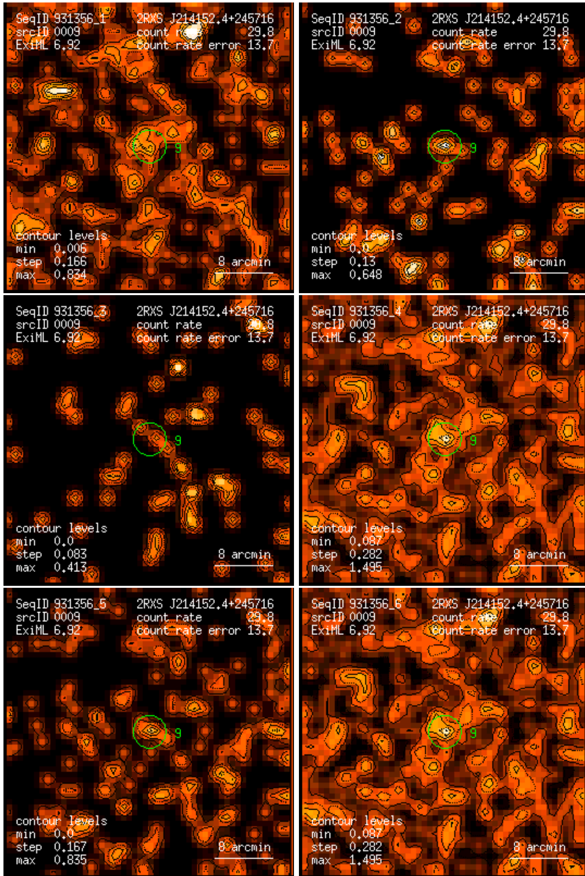
Figure 9: RASS 931356: detection 0009: band rate images, Gaussian filter: (1) PSPC channels 11 – 41, (2) 52 – 90, (3) 91 – 201, (4) 11 – 235, (5) 52 – 201, (6) 11 – 201. Broad band rates in counts/ks. Band rate contour levels in counts/ks/arcmin 2 .
