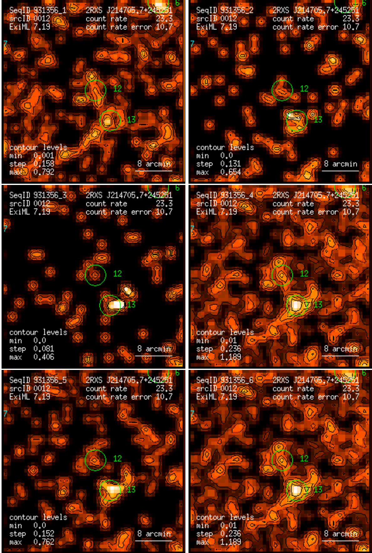
Figure 12: RASS 931356: detection 0012: band rate images, Gaussian filter: (1) PSPC channels 11 – 41, (2) 52 – 90, (3) 91 – 201, (4) 11 – 235, (5) 52 – 201, (6) 11 – 201. Broad band rates in counts/ks. Band rate contour levels in counts/ks/arcmin 2 .
