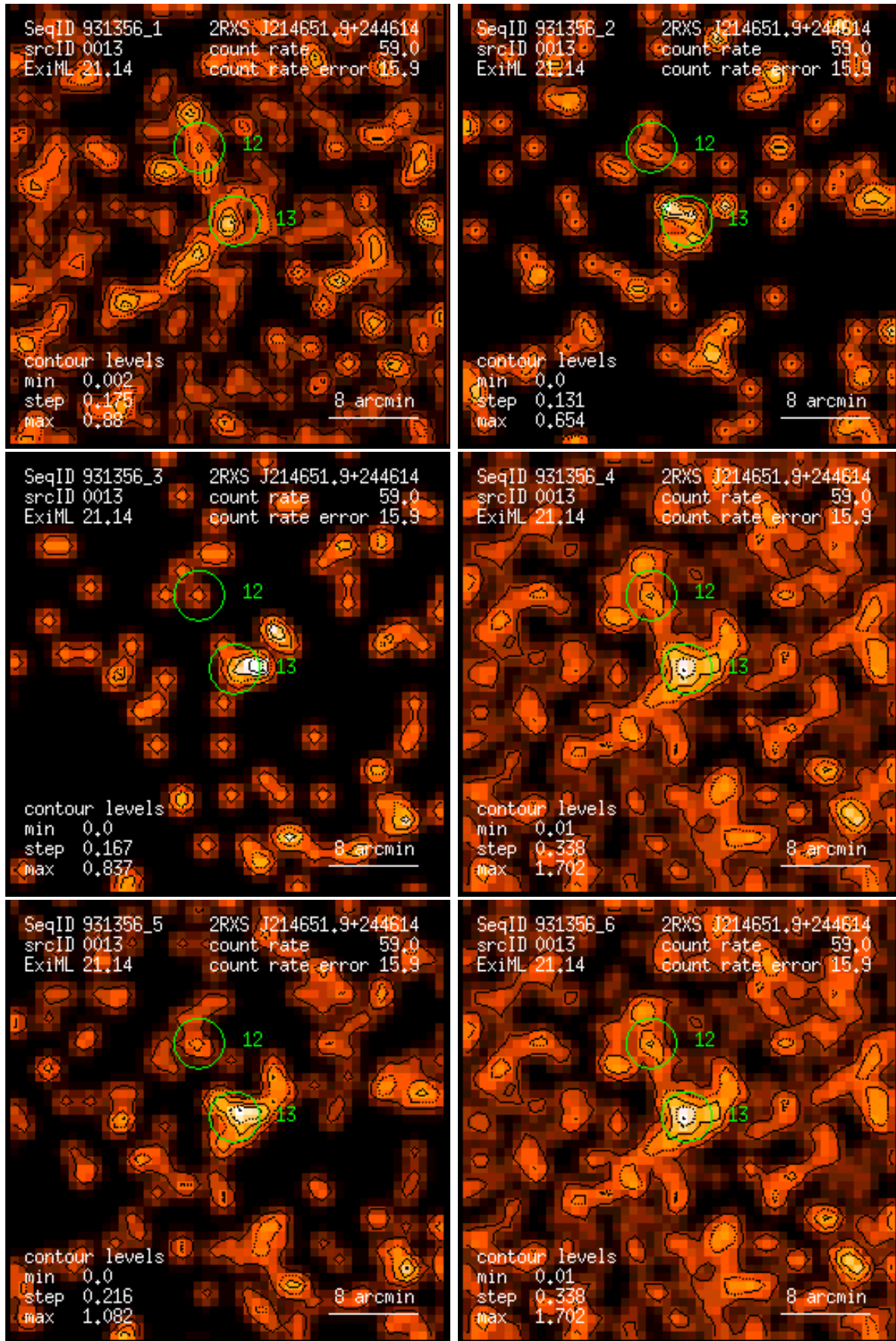
Figure 13: RASS 931356: detection 0013: band rate images, Gaussian filter: (1) PSPC channels 11 – 41, (2) 52 – 90, (3) 91 – 201, (4) 11 – 235, (5) 52 – 201, (6) 11 – 201. Broad band rates in counts/ks. Band rate contour levels in counts/ks/arcmin 2 .
