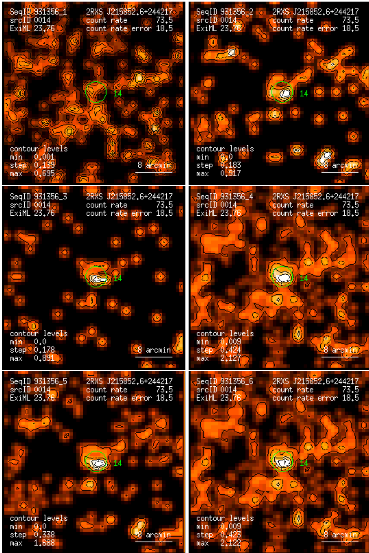
Figure 14: RASS 931356: detection 0014: band rate images, Gaussian filter: (1) PSPC channels 11 – 41, (2) 52 – 90, (3) 91 – 201, (4) 11 – 235, (5) 52 – 201, (6) 11 – 201. Broad band rates in counts/ks. Band rate contour levels in counts/ks/arcmin 2 .
