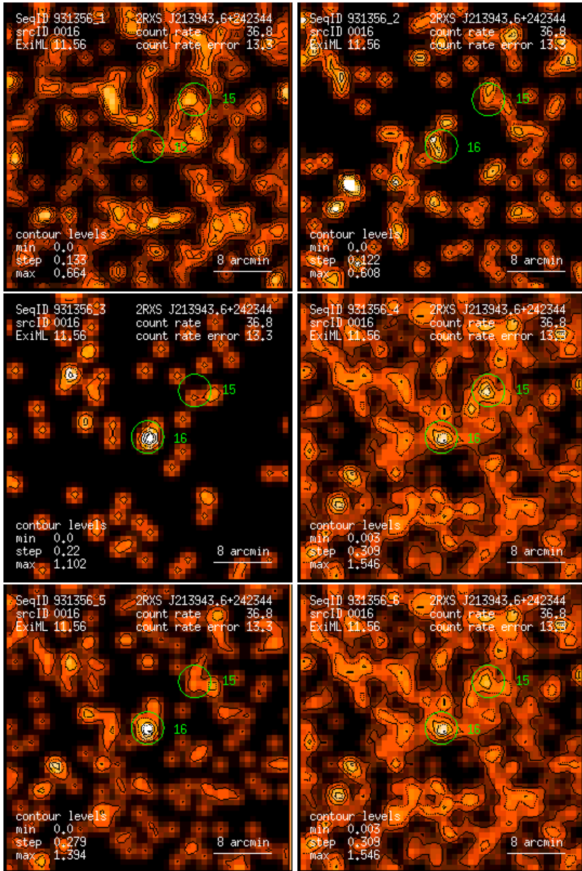
Figure 16: RASS 931356: detection 0016: band rate images, Gaussian filter: (1) PSPC channels 11 – 41, (2) 52 – 90, (3) 91 – 201, (4) 11 – 235, (5) 52 – 201, (6) 11 – 201. Broad band rates in counts/ks. Band rate contour levels in counts/ks/arcmin 2 .
