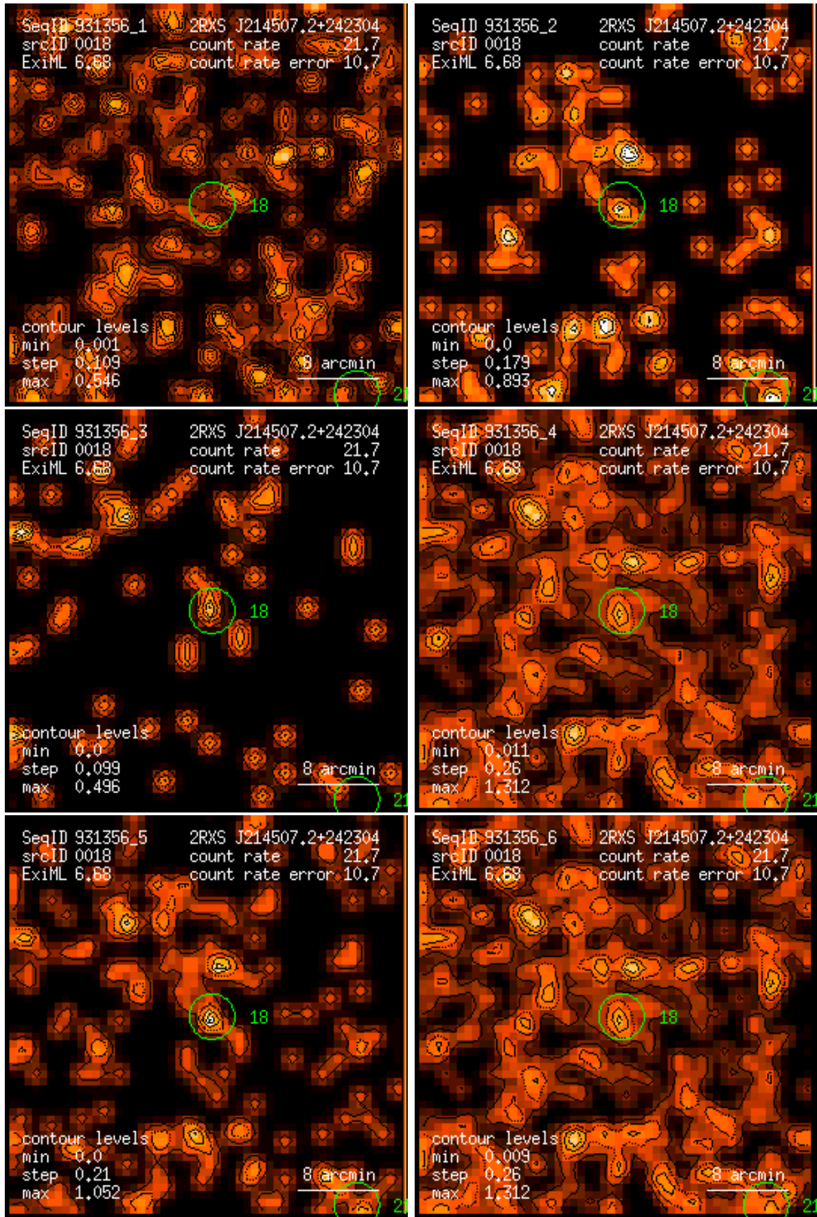
Figure 18: RASS 931356: detection 0018: band rate images, Gaussian filter: (1) PSPC channels 11 – 41, (2) 52 – 90, (3) 91 – 201, (4) 11 – 235, (5) 52 – 201, (6) 11 – 201. Broad band rates in counts/ks. Band rate contour levels in counts/ks/arcmin 2 .
