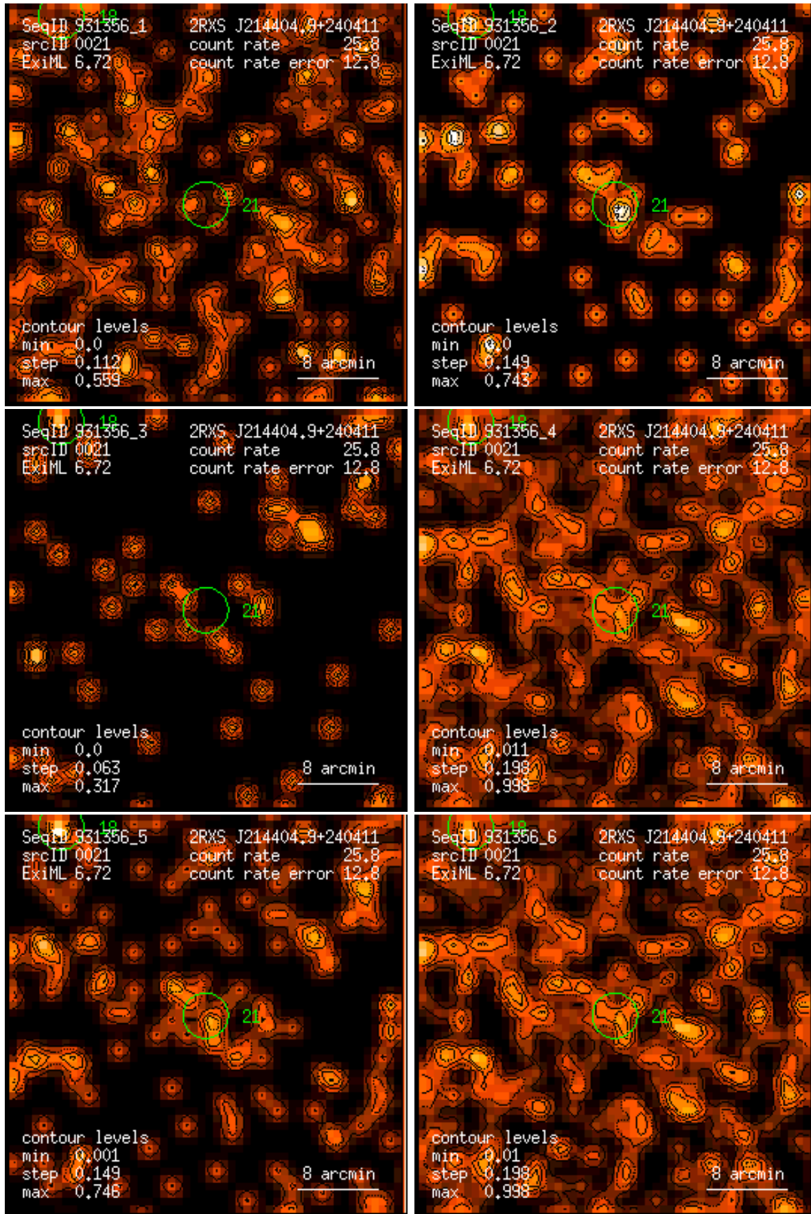
Figure 21: RASS 931356: detection 0021: band rate images, Gaussian filter: (1) PSPC channels 11 – 41, (2) 52 – 90, (3) 91 – 201, (4) 11 – 235, (5) 52 – 201, (6) 11 – 201. Broad band rates in counts/ks. Band rate contour levels in counts/ks/arcmin 2 .
