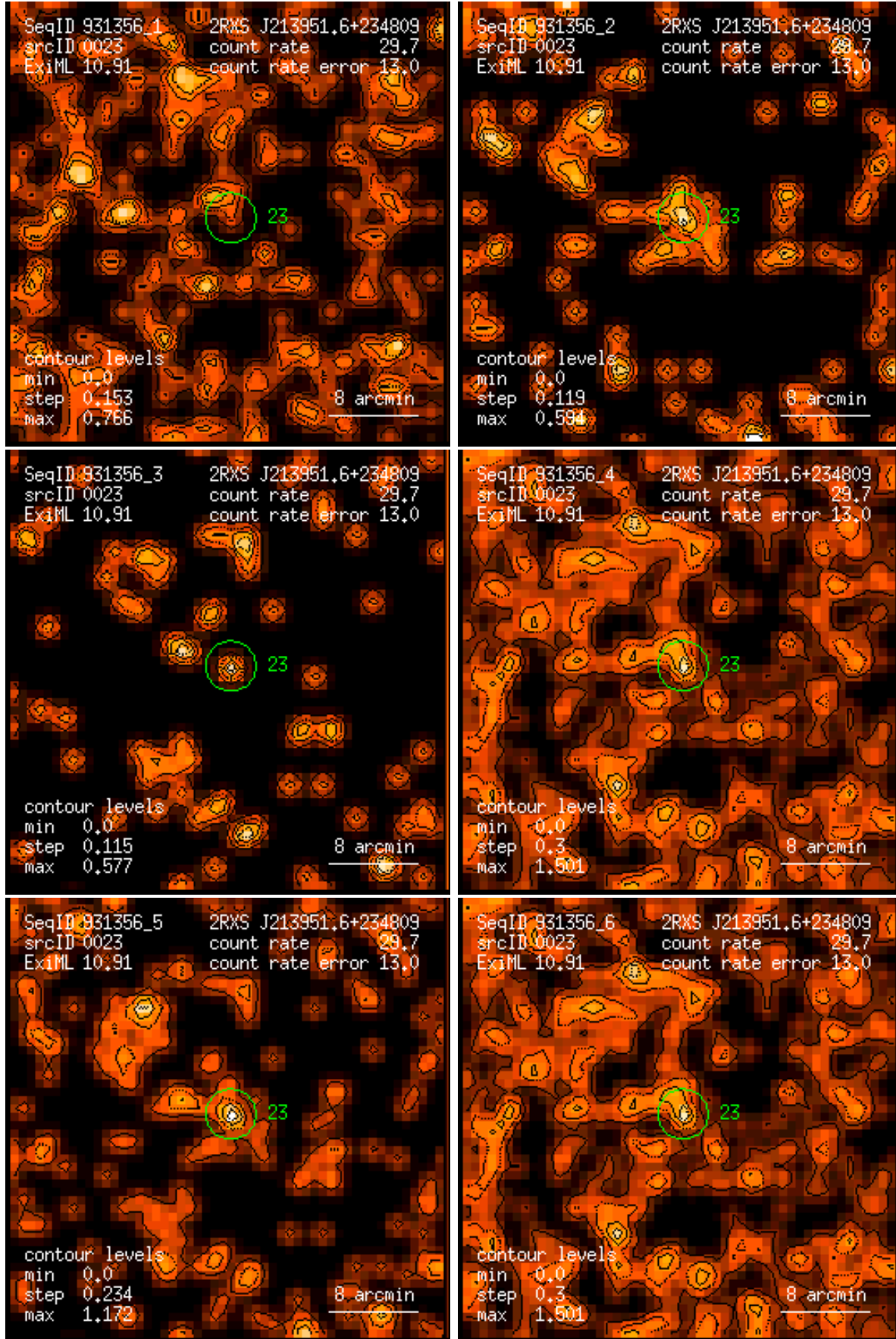
Figure 23: RASS 931356: detection 0023: band rate images, Gaussian filter: (1) PSPC channels 11 – 41, (2) 52 – 90, (3) 91 – 201, (4) 11 – 235, (5) 52 – 201, (6) 11 – 201. Broad band rates in counts/ks. Band rate contour levels in counts/ks/arcmin 2 .
