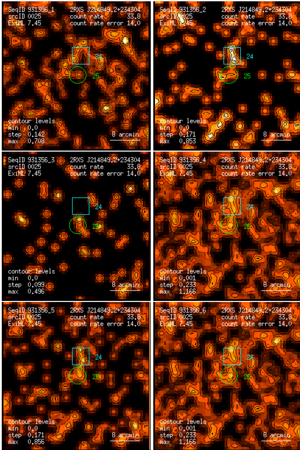
Figure 25: RASS 931356: detection 0025: band rate images, Gaussian filter: (1) PSPC channels 11 – 41, (2) 52 – 90, (3) 91 – 201, (4) 11 – 235, (5) 52 – 201, (6) 11 – 201. Broad band rates in counts/ks. Band rate contour levels in counts/ks/arcmin 2 .
