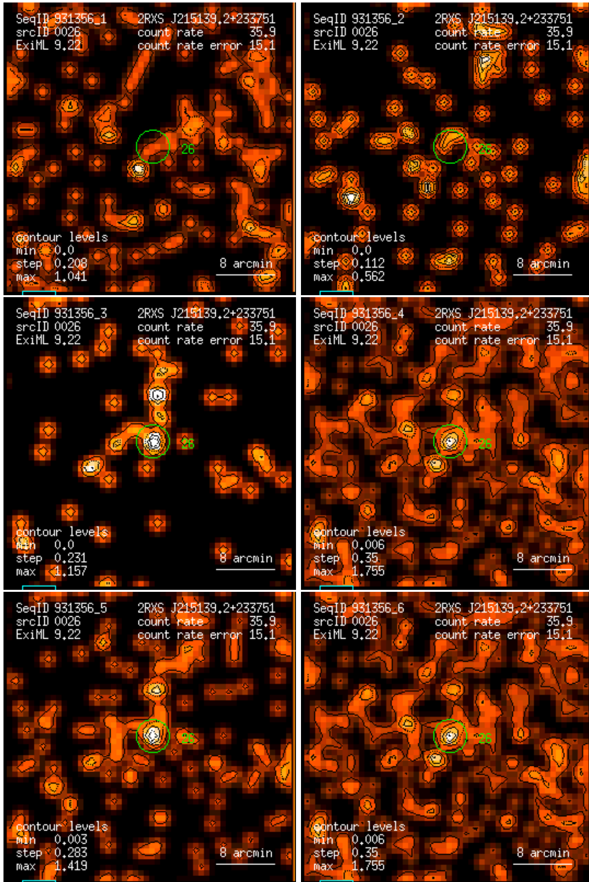
Figure 26: RASS 931356: detection 0026: band rate images, Gaussian filter: (1) PSPC channels 11 – 41, (2) 52 – 90, (3) 91 – 201, (4) 11 – 235, (5) 52 – 201, (6) 11 – 201. Broad band rates in counts/ks. Band rate contour levels in counts/ks/arcmin 2 .
