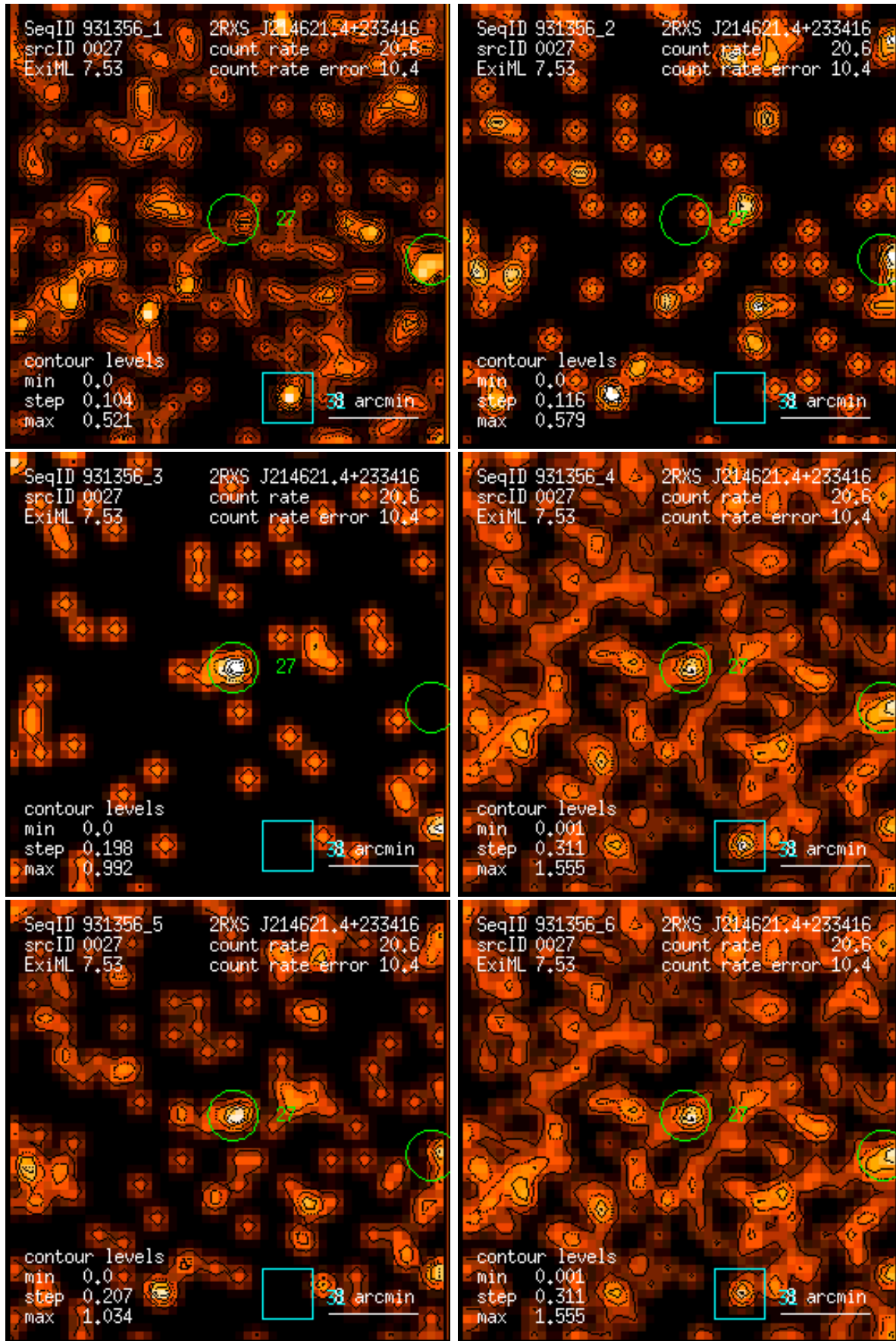
Figure 27: RASS 931356: detection 0027: band rate images, Gaussian filter: (1) PSPC channels 11 – 41, (2) 52 – 90, (3) 91 – 201, (4) 11 – 235, (5) 52 – 201, (6) 11 – 201. Broad band rates in counts/ks. Band rate contour levels in counts/ks/arcmin 2 .
