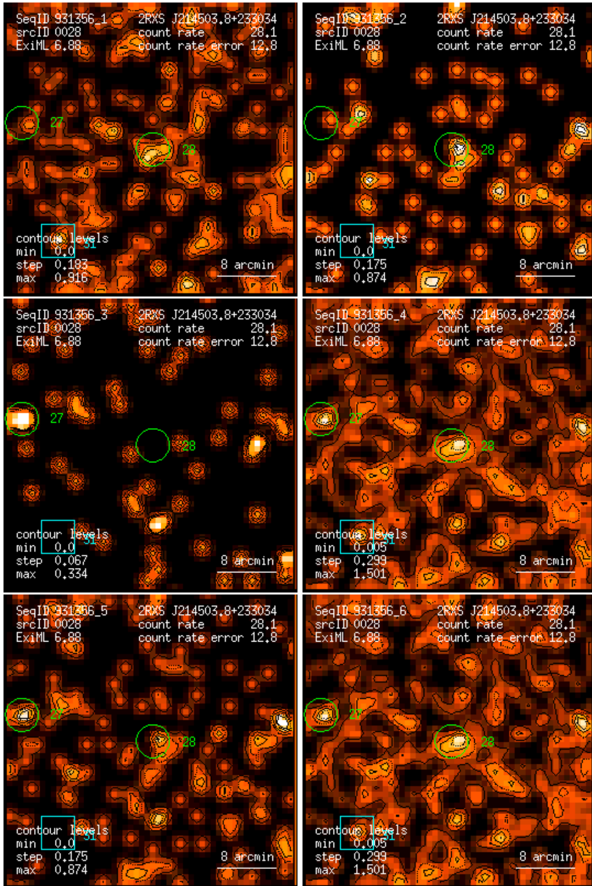
Figure 28: RASS 931356: detection 0028: band rate images, Gaussian filter: (1) PSPC channels 11 – 41, (2) 52 – 90, (3) 91 – 201, (4) 11 – 235, (5) 52 – 201, (6) 11 – 201. Broad band rates in counts/ks. Band rate contour levels in counts/ks/arcmin 2 .
