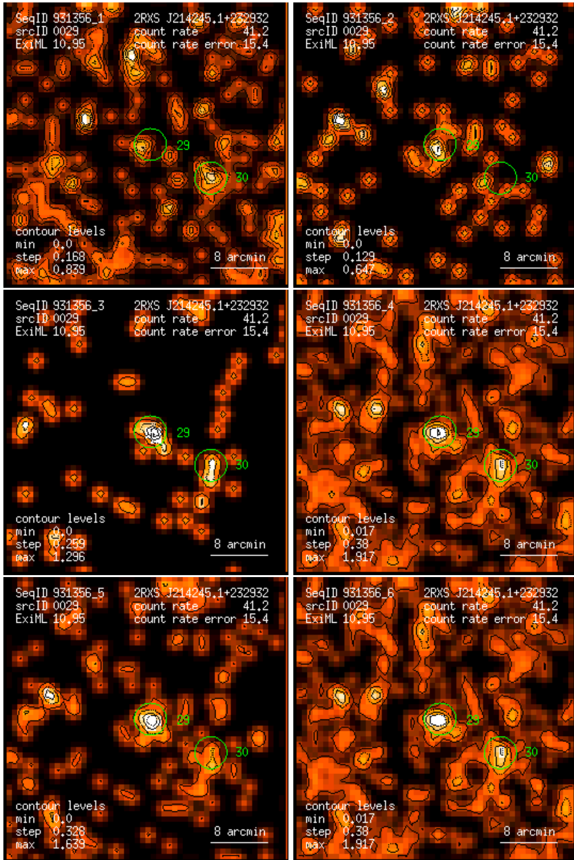
Figure 29: RASS 931356: detection 0029: band rate images, Gaussian filter: (1) PSPC channels 11 – 41, (2) 52 – 90, (3) 91 – 201, (4) 11 – 235, (5) 52 – 201, (6) 11 – 201. Broad band rates in counts/ks. Band rate contour levels in counts/ks/arcmin 2 .
