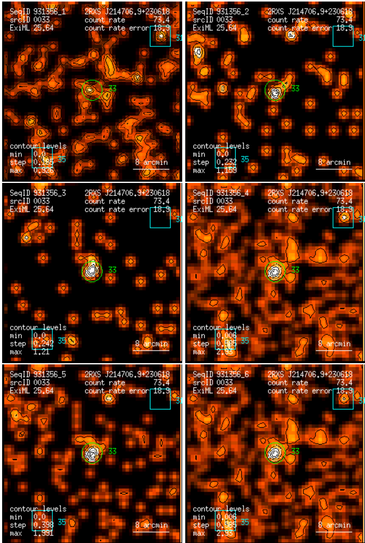
Figure 33: RASS 931356: detection 0033: band rate images, Gaussian filter: (1) PSPC channels 11 – 41, (2) 52 – 90, (3) 91 – 201, (4) 11 – 235, (5) 52 – 201, (6) 11 – 201. Broad band rates in counts/ks. Band rate contour levels in counts/ks/arcmin 2 .
