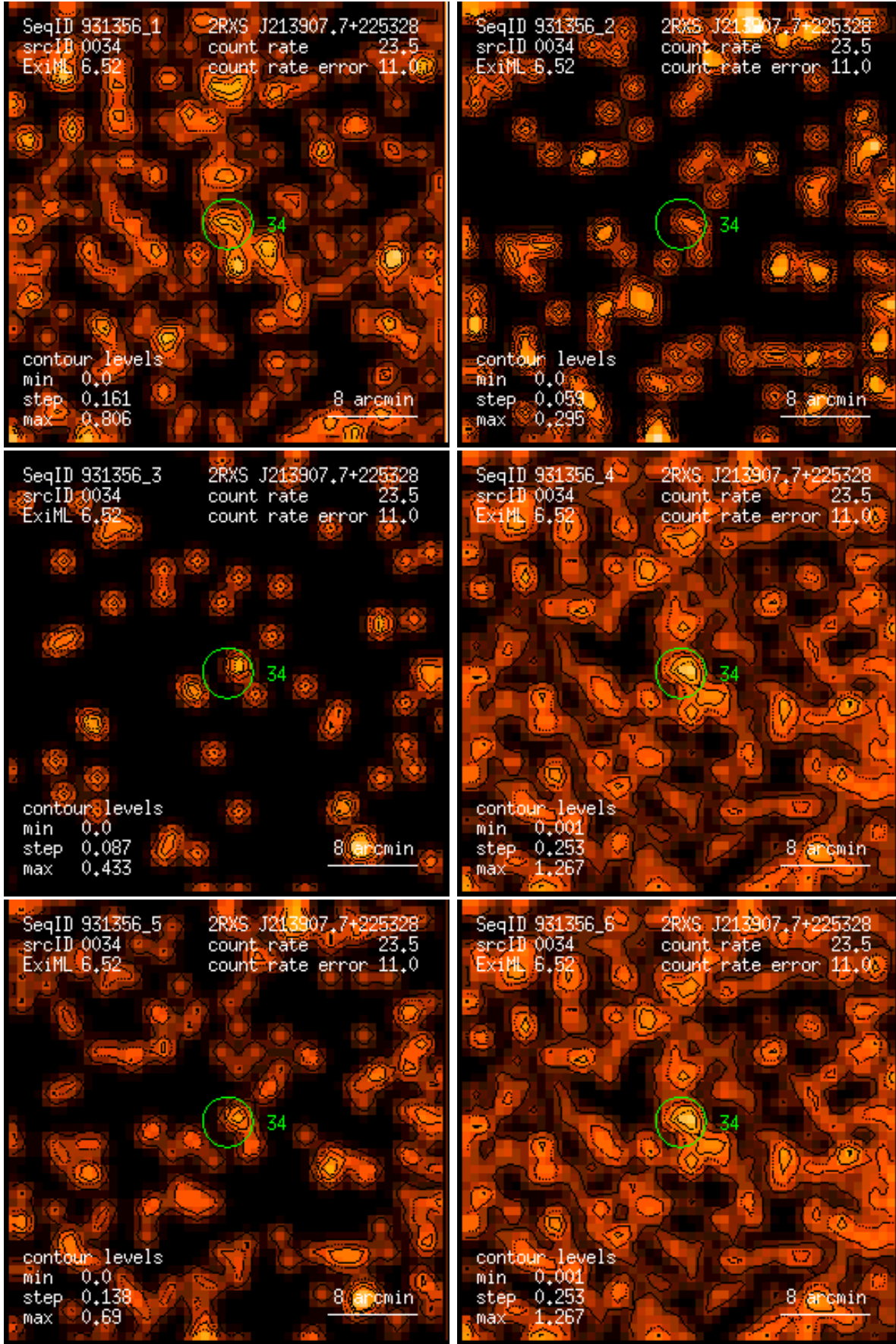
Figure 34: RASS 931356: detection 0034: band rate images, Gaussian filter: (1) PSPC channels 11 – 41, (2) 52 – 90, (3) 91 – 201, (4) 11 – 235, (5) 52 – 201, (6) 11 – 201. Broad band rates in counts/ks. Band rate contour levels in counts/ks/arcmin 2 .
