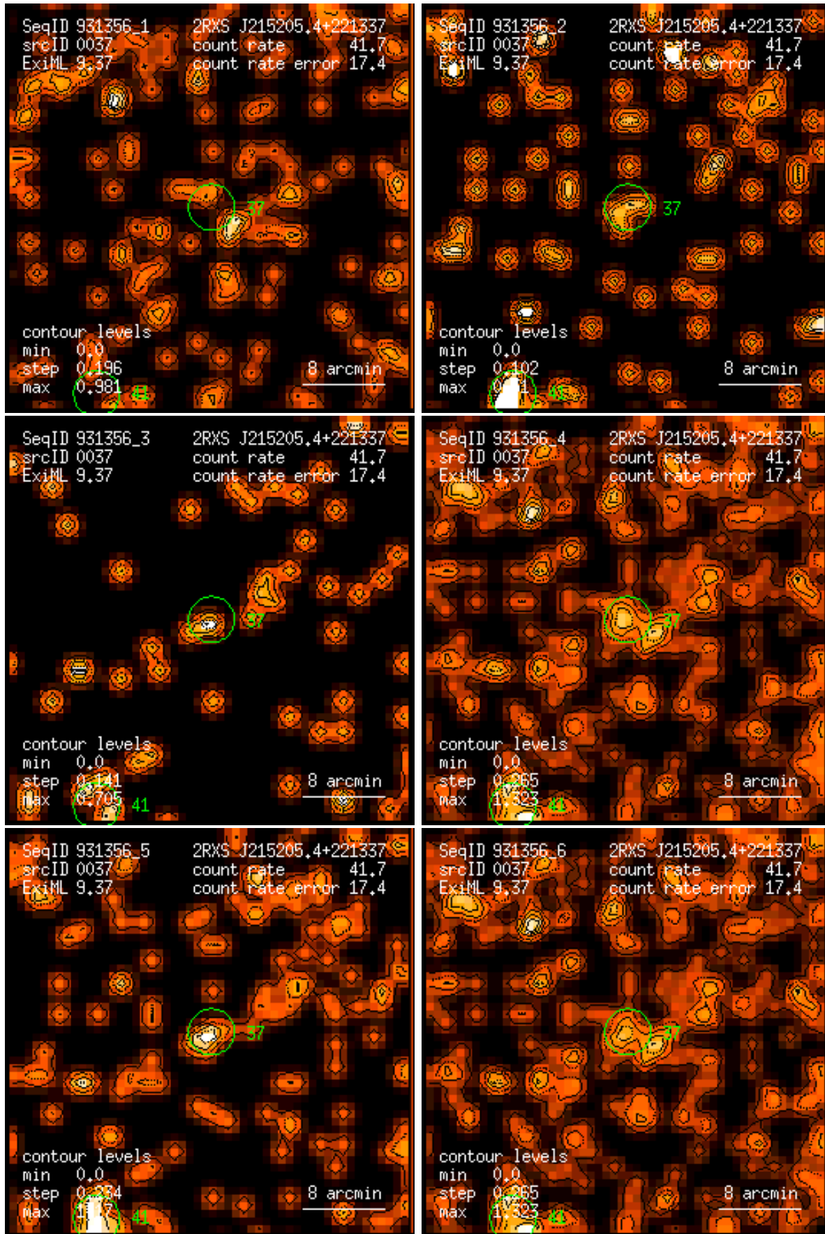
Figure 37: RASS 931356: detection 0037: band rate images, Gaussian filter: (1) PSPC channels 11 – 41, (2) 52 – 90, (3) 91 – 201, (4) 11 – 235, (5) 52 – 201, (6) 11 – 201. Broad band rates in counts/ks. Band rate contour levels in counts/ks/arcmin 2 .
