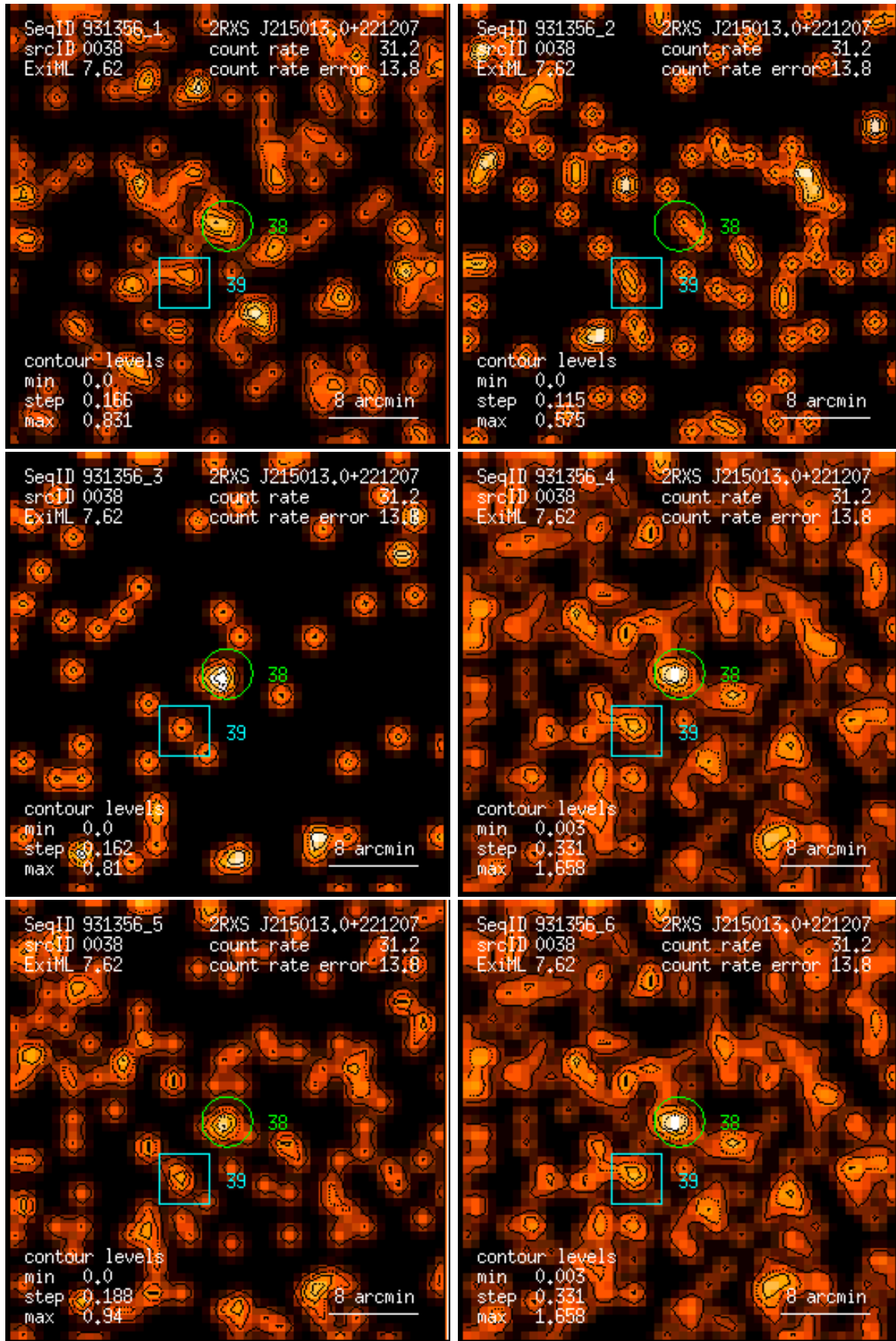
Figure 38: RASS 931356: detection 0038: band rate images, Gaussian filter: (1) PSPC channels 11 – 41, (2) 52 – 90, (3) 91 – 201, (4) 11 – 235, (5) 52 – 201, (6) 11 – 201. Broad band rates in counts/ks. Band rate contour levels in counts/ks/arcmin 2 .
