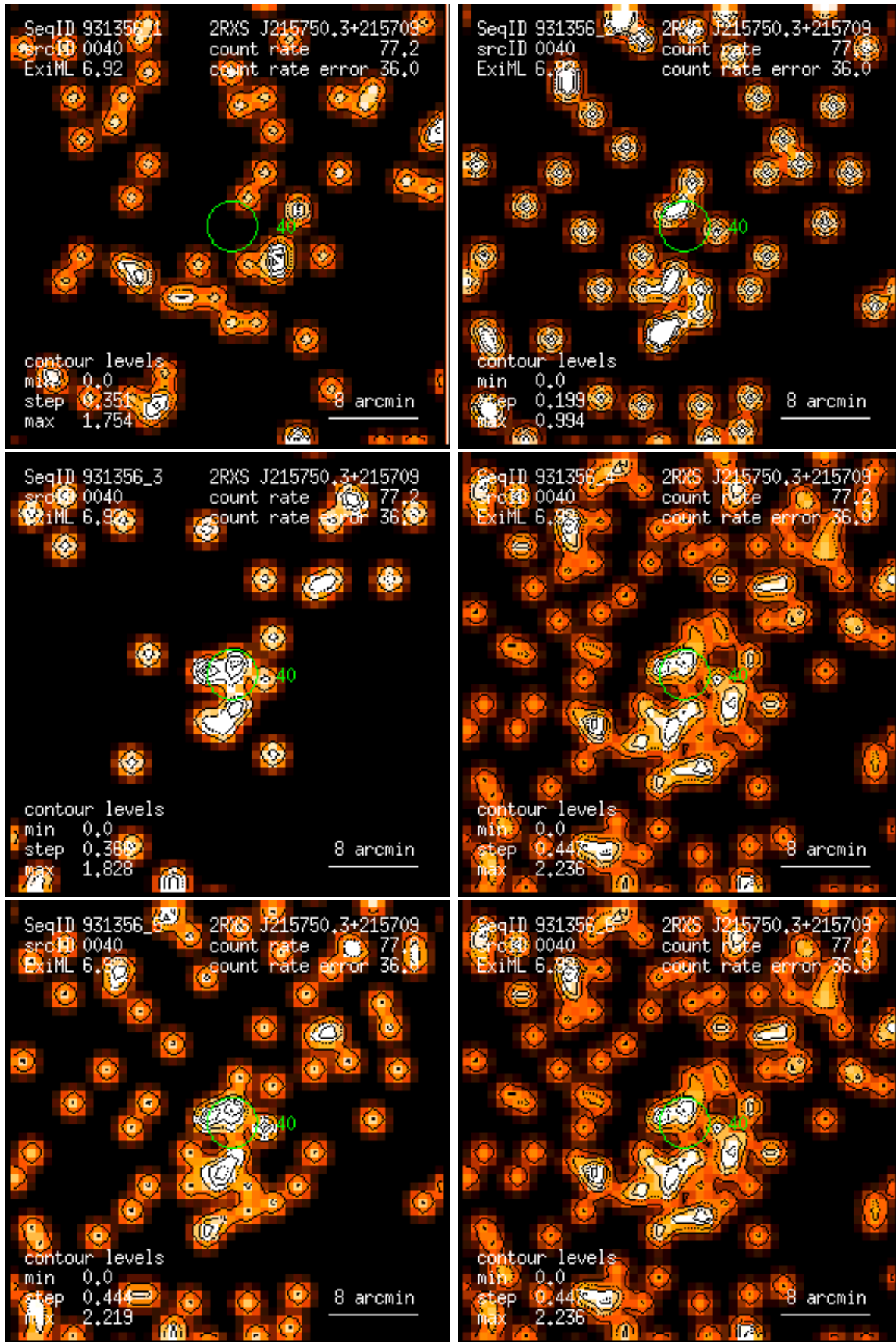
Figure 40: RASS 931356: detection 0040: band rate images, Gaussian filter: (1) PSPC channels 11 – 41, (2) 52 – 90, (3) 91 – 201, (4) 11 – 235, (5) 52 – 201, (6) 11 – 201. Broad band rates in counts/ks. Band rate contour levels in counts/ks/arcmin 2 .
