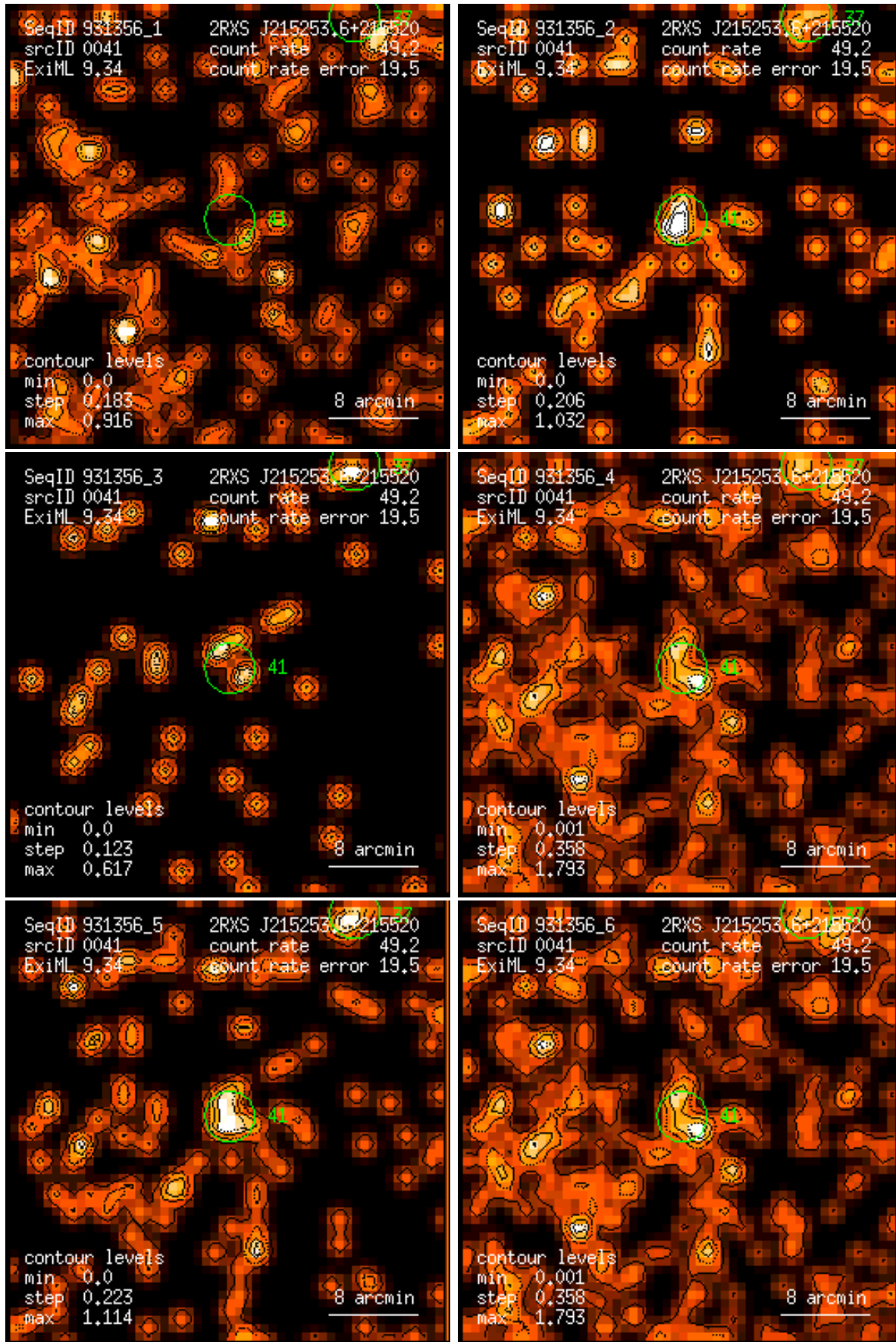
Figure 41: RASS 931356: detection 0041: band rate images, Gaussian filter: (1) PSPC channels 11 – 41, (2) 52 – 90, (3) 91 – 201, (4) 11 – 235, (5) 52 – 201, (6) 11 – 201. Broad band rates in counts/ks. Band rate contour levels in counts/ks/arcmin 2 .
