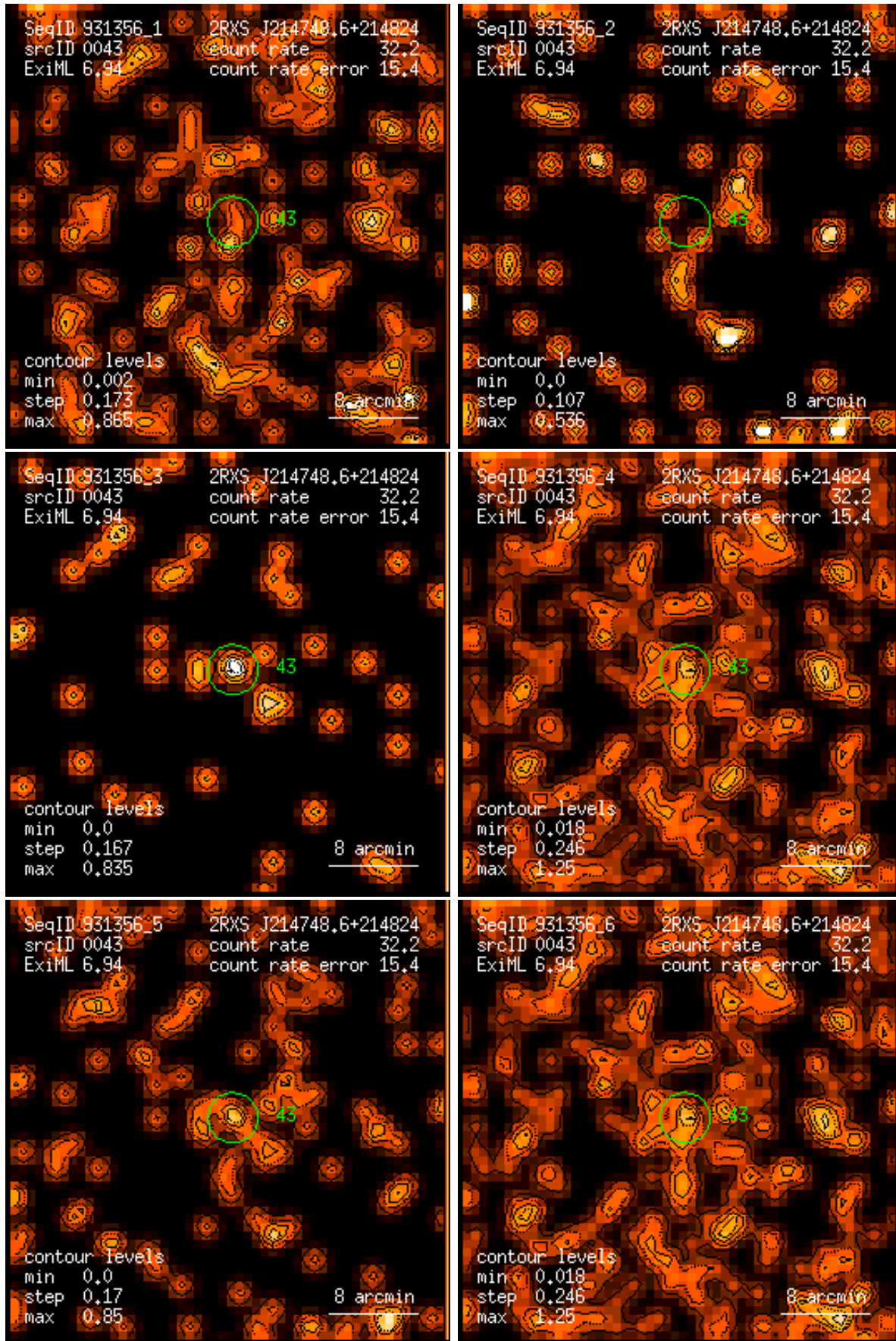
Figure 43: RASS 931356: detection 0043: band rate images, Gaussian filter: (1) PSPC channels 11 – 41, (2) 52 – 90, (3) 91 – 201, (4) 11 – 235, (5) 52 – 201, (6) 11 – 201. Broad band rates in counts/ks. Band rate contour levels in counts/ks/arcmin 2 .
