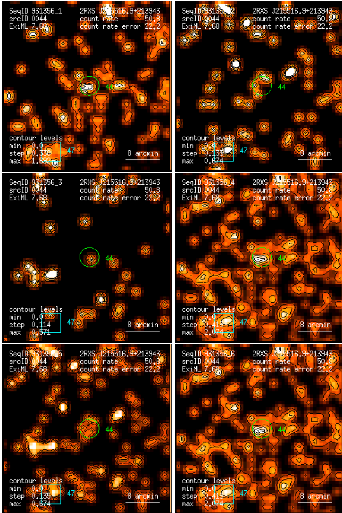
Figure 44: RASS 931356: detection 0044: band rate images, Gaussian filter: (1) PSPC channels 11 – 41, (2) 52 – 90, (3) 91 – 201, (4) 11 – 235, (5) 52 – 201, (6) 11 – 201. Broad band rates in counts/ks. Band rate contour levels in counts/ks/arcmin 2 .
