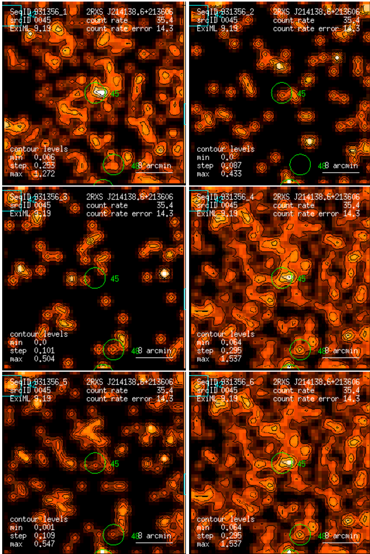
Figure 45: RASS 931356: detection 0045: band rate images, Gaussian filter: (1) PSPC channels 11 – 41, (2) 52 – 90, (3) 91 – 201, (4) 11 – 235, (5) 52 – 201, (6) 11 – 201. Broad band rates in counts/ks. Band rate contour levels in counts/ks/arcmin 2 .
