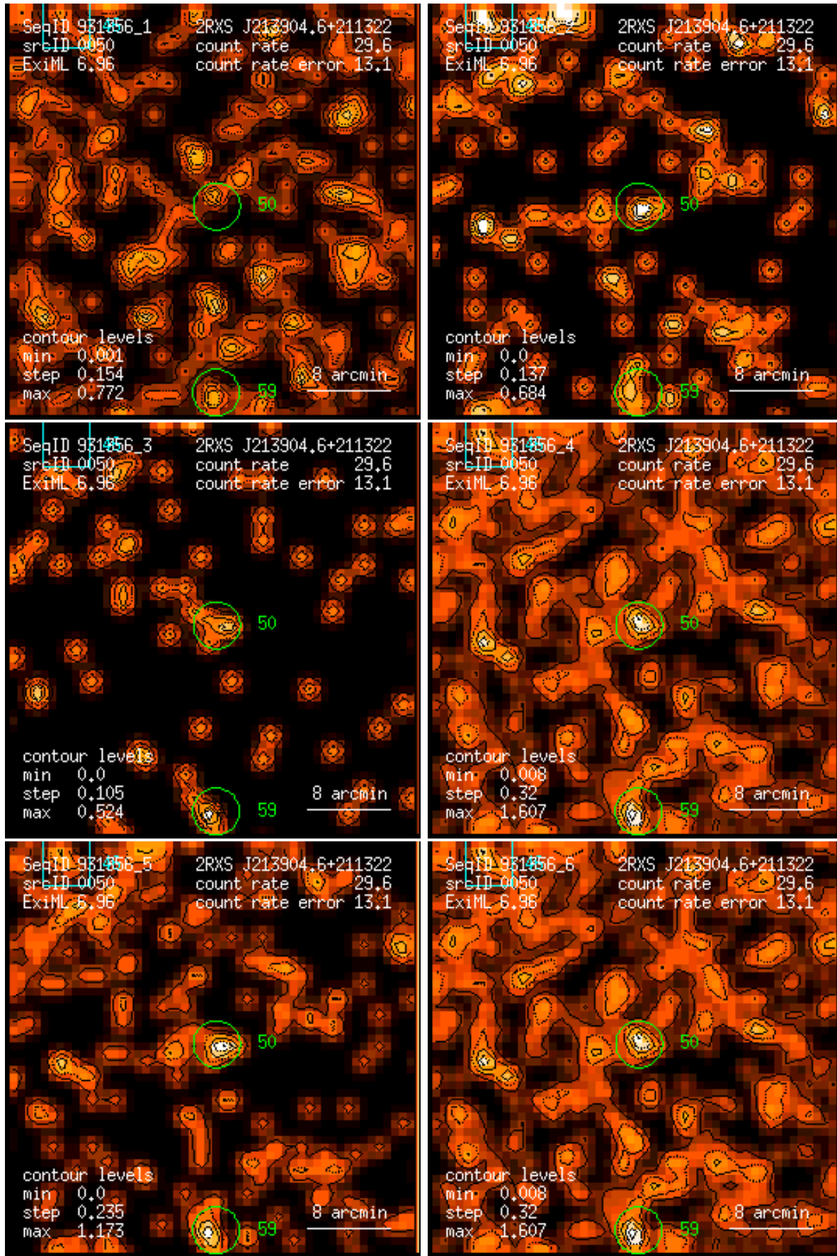
Figure 50: RASS 931356: detection 0050: band rate images, Gaussian filter: (1) PSPC channels 11 – 41, (2) 52 – 90, (3) 91 – 201, (4) 11 – 235, (5) 52 – 201, (6) 11 – 201. Broad band rates in counts/ks. Band rate contour levels in counts/ks/arcmin 2 .
