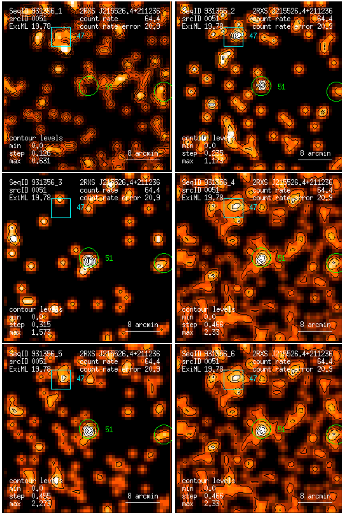
Figure 51: RASS 931356: detection 0051: band rate images, Gaussian filter: (1) PSPC channels 11 – 41, (2) 52 – 90, (3) 91 – 201, (4) 11 – 235, (5) 52 – 201, (6) 11 – 201. Broad band rates in counts/ks. Band rate contour levels in counts/ks/arcmin 2 .
