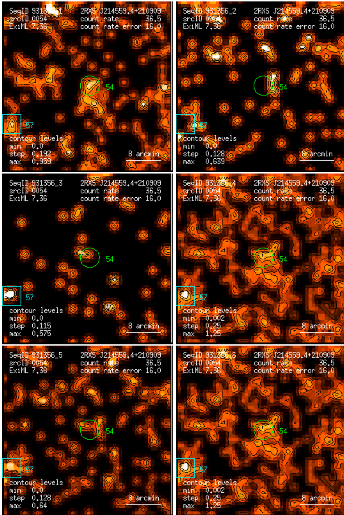
Figure 54: RASS 931356: detection 0054: band rate images, Gaussian filter: (1) PSPC channels 11 – 41, (2) 52 – 90, (3) 91 – 201, (4) 11 – 235, (5) 52 – 201, (6) 11 – 201. Broad band rates in counts/ks. Band rate contour levels in counts/ks/arcmin 2 .
