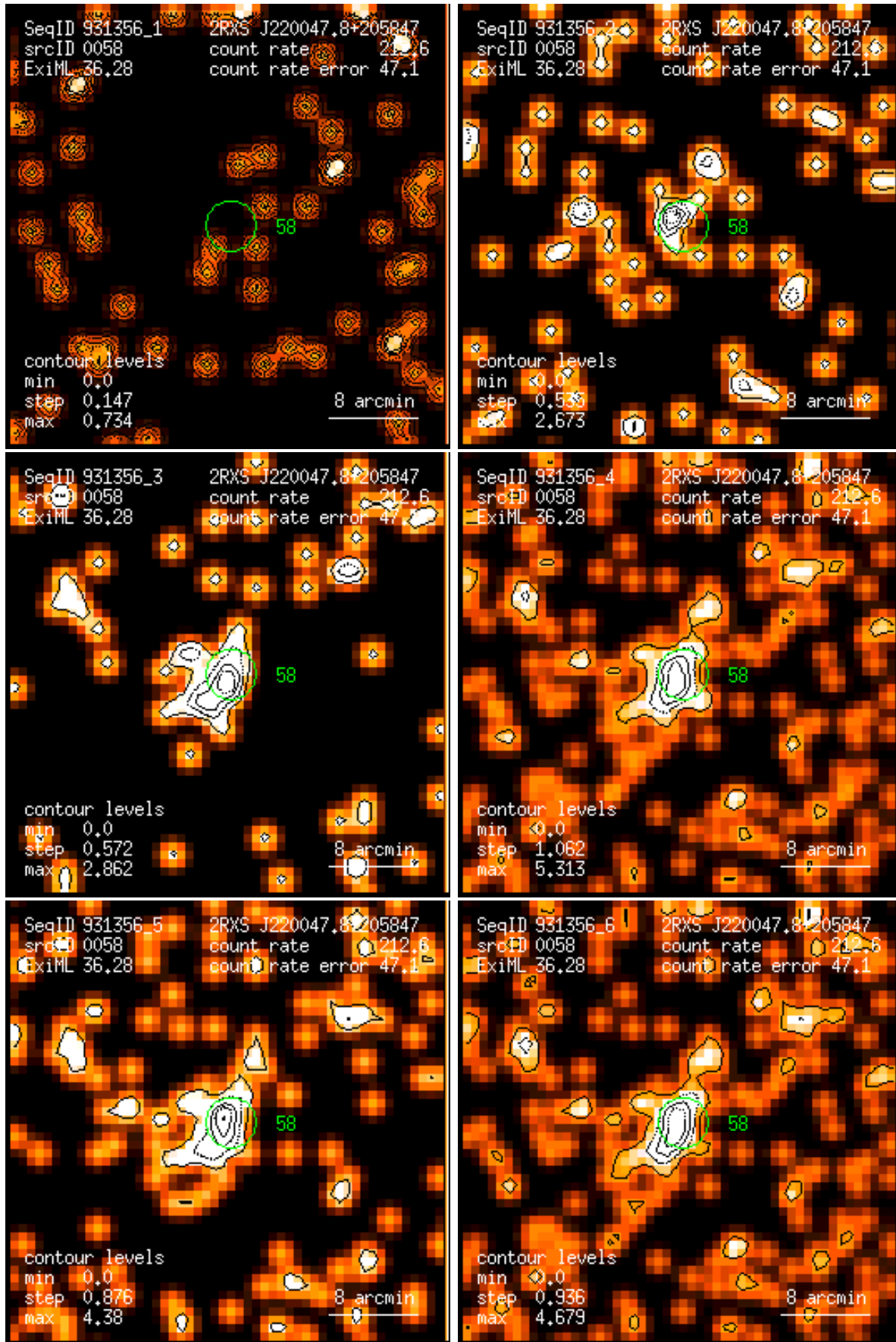
Figure 58: RASS 931356: detection 0058: band rate images, Gaussian filter: (1) PSPC channels 11 – 41, (2) 52 – 90, (3) 91 – 201, (4) 11 – 235, (5) 52 – 201, (6) 11 – 201. Broad band rates in counts/ks. Band rate contour levels in counts/ks/arcmin 2 .
