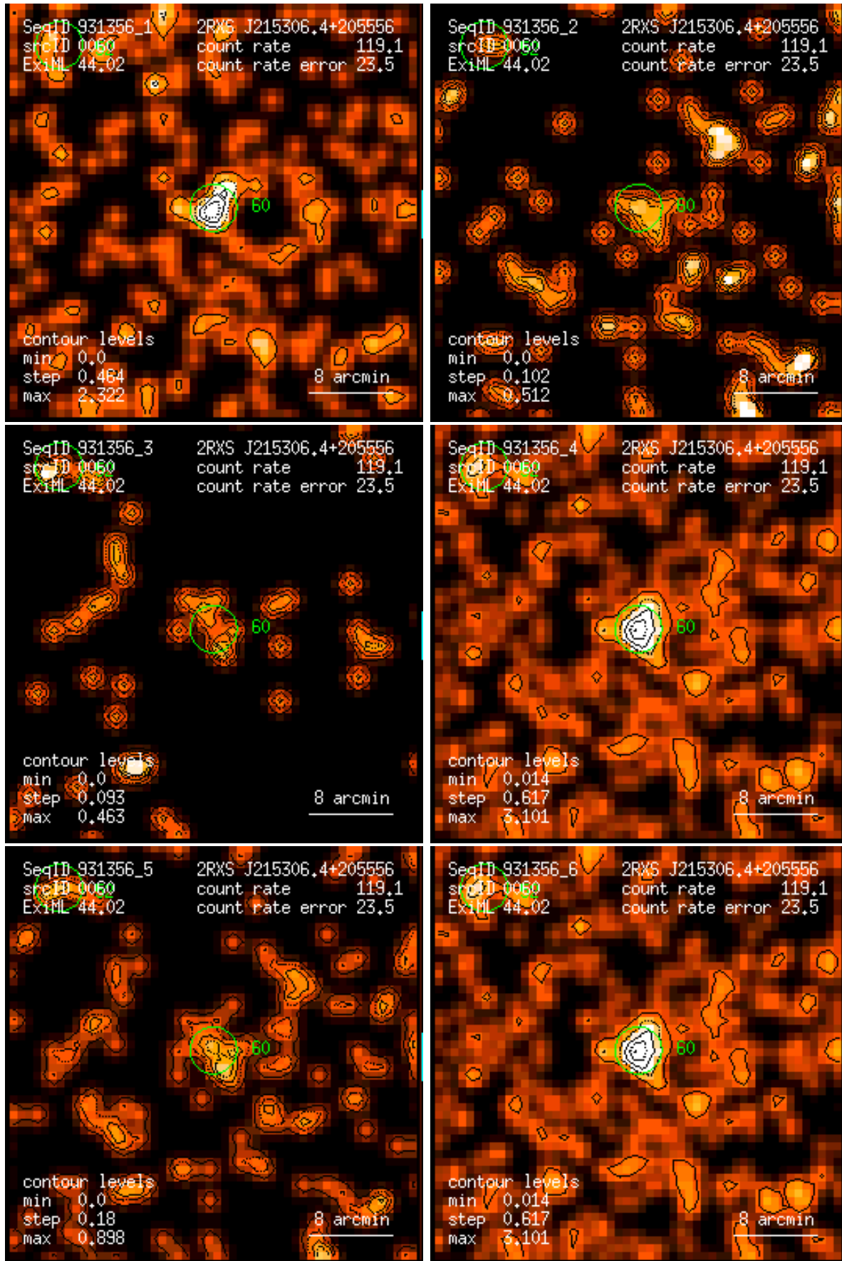
Figure 60: RASS 931356: detection 0060: band rate images, Gaussian filter: (1) PSPC channels 11 – 41, (2) 52 – 90, (3) 91 – 201, (4) 11 – 235, (5) 52 – 201, (6) 11 – 201. Broad band rates in counts/ks. Band rate contour levels in counts/ks/arcmin 2 .
