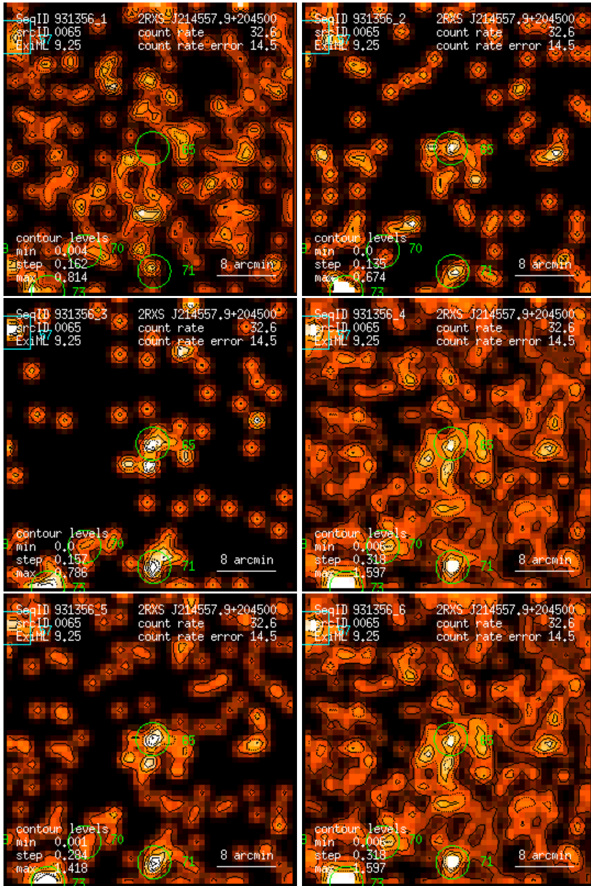
Figure 65: RASS 931356: detection 0065: band rate images, Gaussian filter: (1) PSPC channels 11 – 41, (2) 52 – 90, (3) 91 – 201, (4) 11 – 235, (5) 52 – 201, (6) 11 – 201. Broad band rates in counts/ks. Band rate contour levels in counts/ks/arcmin 2 .
