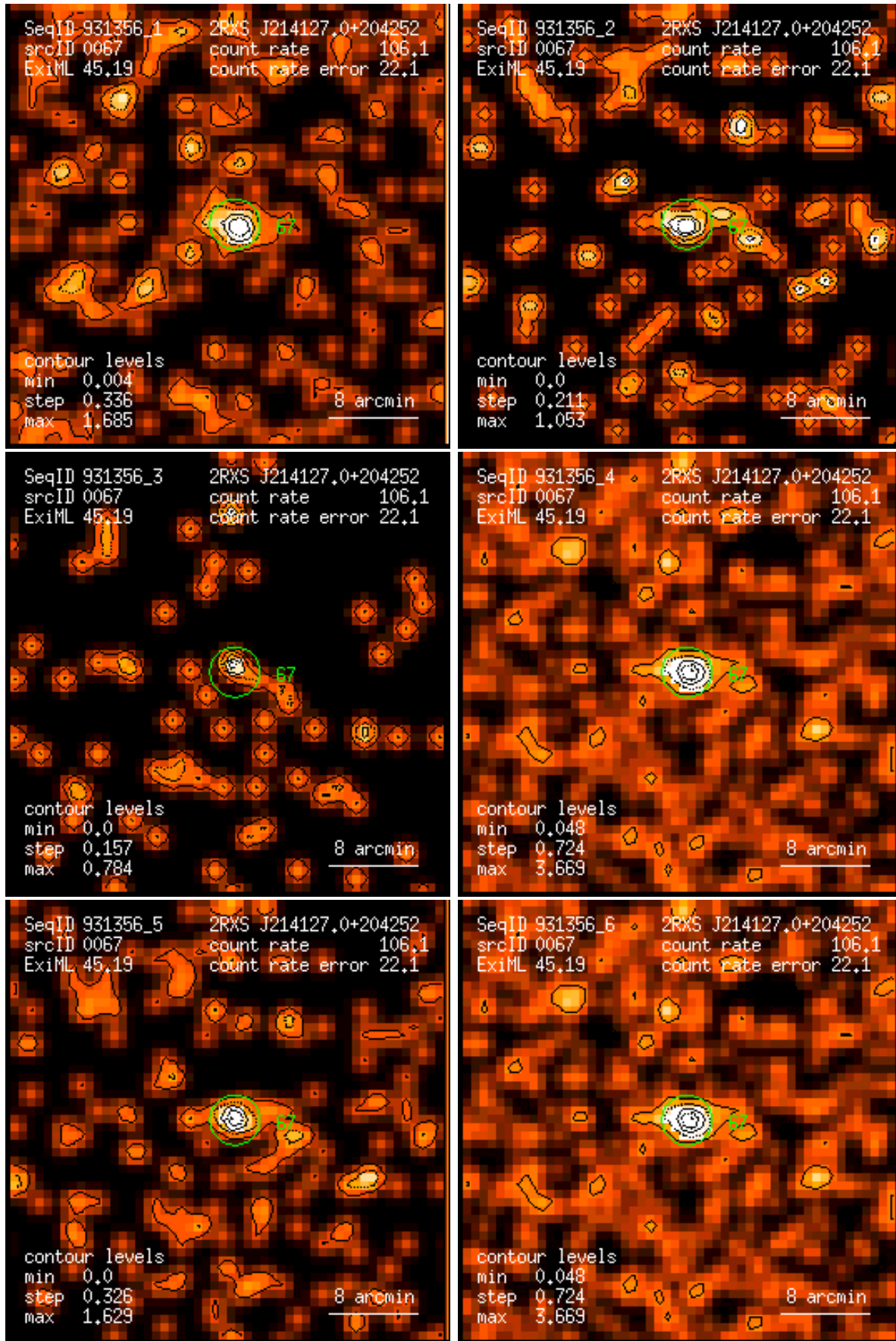
Figure 67: RASS 931356: detection 0067: band rate images, Gaussian filter: (1) PSPC channels 11 – 41, (2) 52 – 90, (3) 91 – 201, (4) 11 – 235, (5) 52 – 201, (6) 11 – 201. Broad band rates in counts/ks. Band rate contour levels in counts/ks/arcmin 2 .
