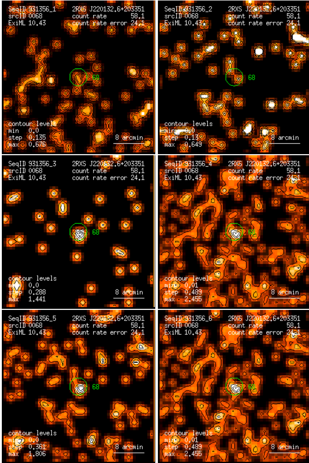
Figure 68: RASS 931356: detection 0068: band rate images, Gaussian filter: (1) PSPC channels 11 – 41, (2) 52 – 90, (3) 91 – 201, (4) 11 – 235, (5) 52 – 201, (6) 11 – 201. Broad band rates in counts/ks. Band rate contour levels in counts/ks/arcmin 2 .
