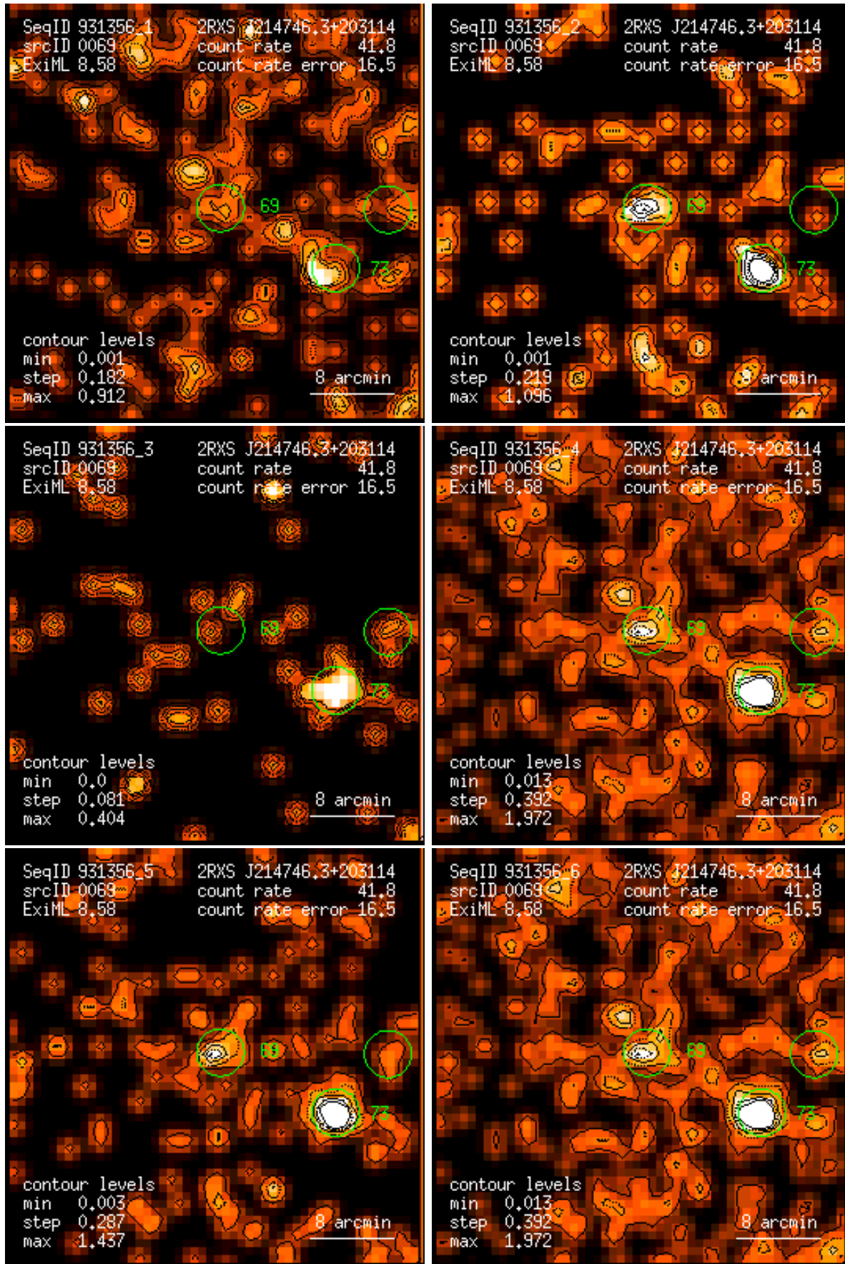
Figure 69: RASS 931356: detection 0069: band rate images, Gaussian filter: (1) PSPC channels 11 – 41, (2) 52 – 90, (3) 91 – 201, (4) 11 – 235, (5) 52 – 201, (6) 11 – 201. Broad band rates in counts/ks. Band rate contour levels in counts/ks/arcmin 2 .
