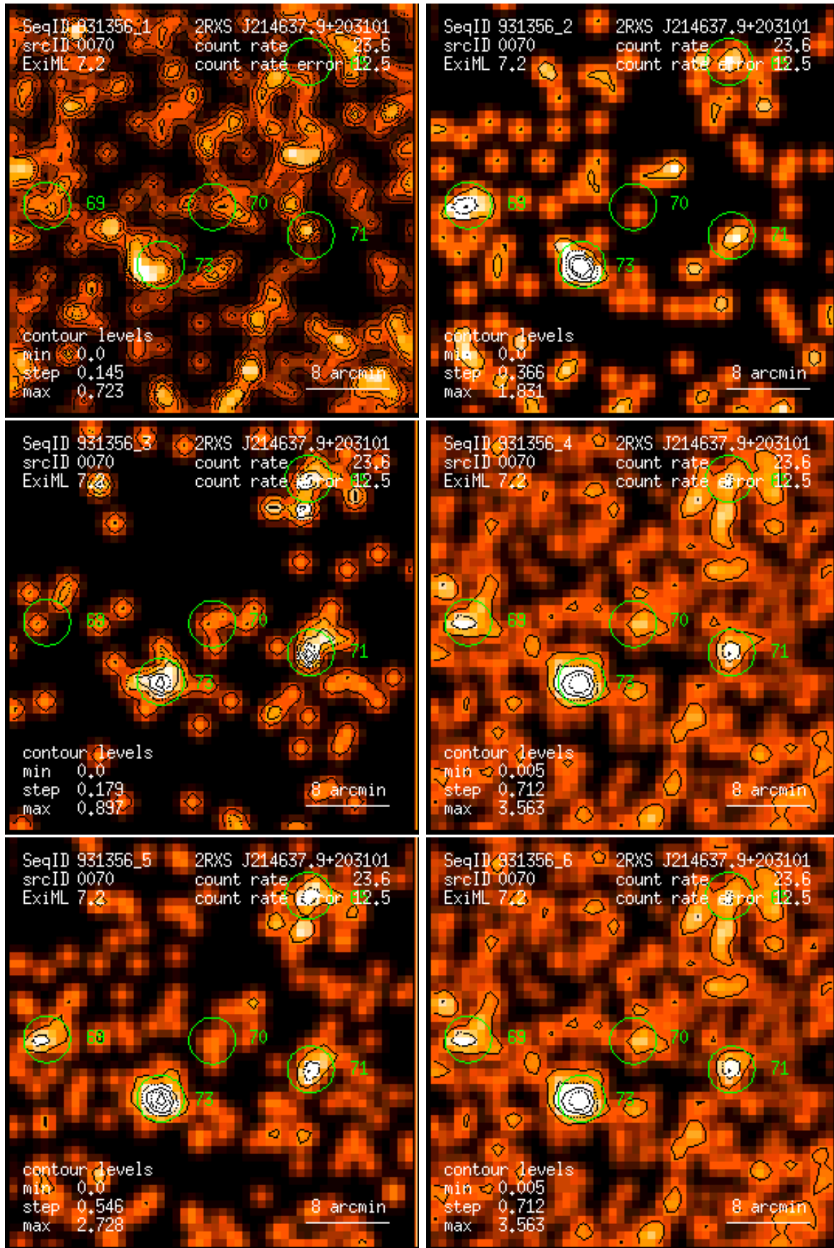
Figure 70: RASS 931356: detection 0070: band rate images, Gaussian filter: (1) PSPC channels 11 – 41, (2) 52 – 90, (3) 91 – 201, (4) 11 – 235, (5) 52 – 201, (6) 11 – 201. Broad band rates in counts/ks. Band rate contour levels in counts/ks/arcmin 2 .
