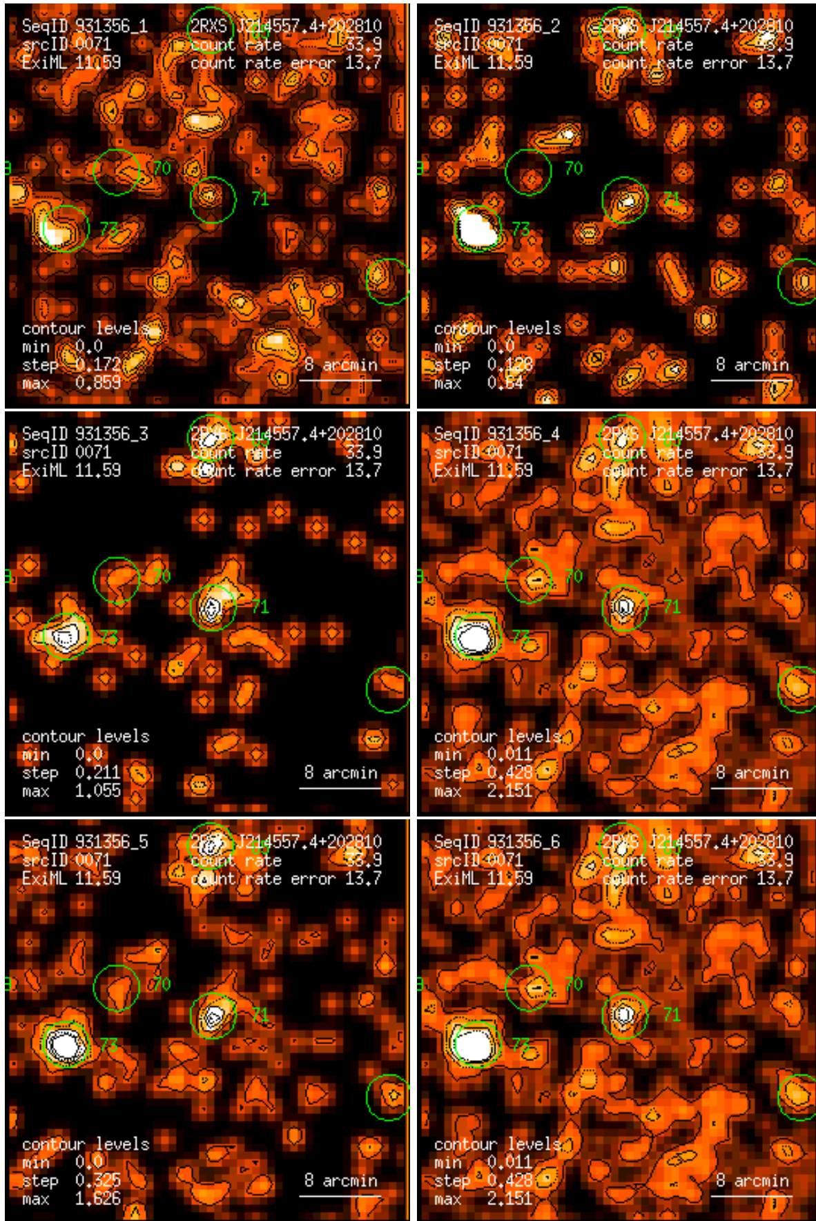
Figure 71: RASS 931356: detection 0071: band rate images, Gaussian filter: (1) PSPC channels 11 – 41, (2) 52 – 90, (3) 91 – 201, (4) 11 – 235, (5) 52 – 201, (6) 11 – 201. Broad band rates in counts/ks. Band rate contour levels in counts/ks/arcmin 2 .
