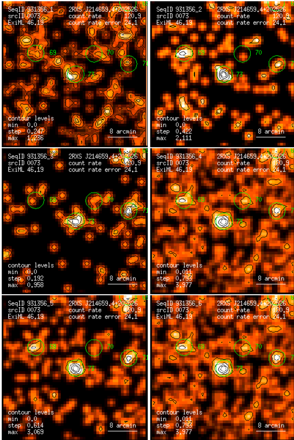
Figure 73: RASS 931356: detection 0073: band rate images, Gaussian filter: (1) PSPC channels 11 – 41, (2) 52 – 90, (3) 91 – 201, (4) 11 – 235, (5) 52 – 201, (6) 11 – 201. Broad band rates in counts/ks. Band rate contour levels in counts/ks/arcmin 2 .
