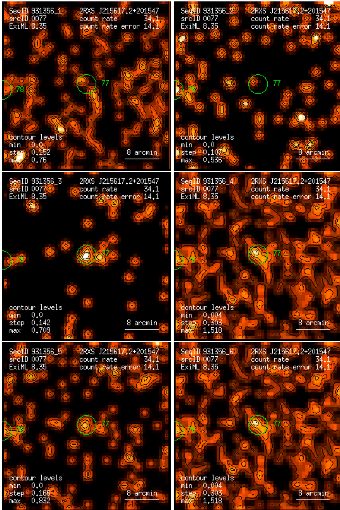
Figure 77: RASS 931356: detection 0077: band rate images, Gaussian filter: (1) PSPC channels 11 – 41, (2) 52 – 90, (3) 91 – 201, (4) 11 – 235, (5) 52 – 201, (6) 11 – 201. Broad band rates in counts/ks. Band rate contour levels in counts/ks/arcmin 2 .
