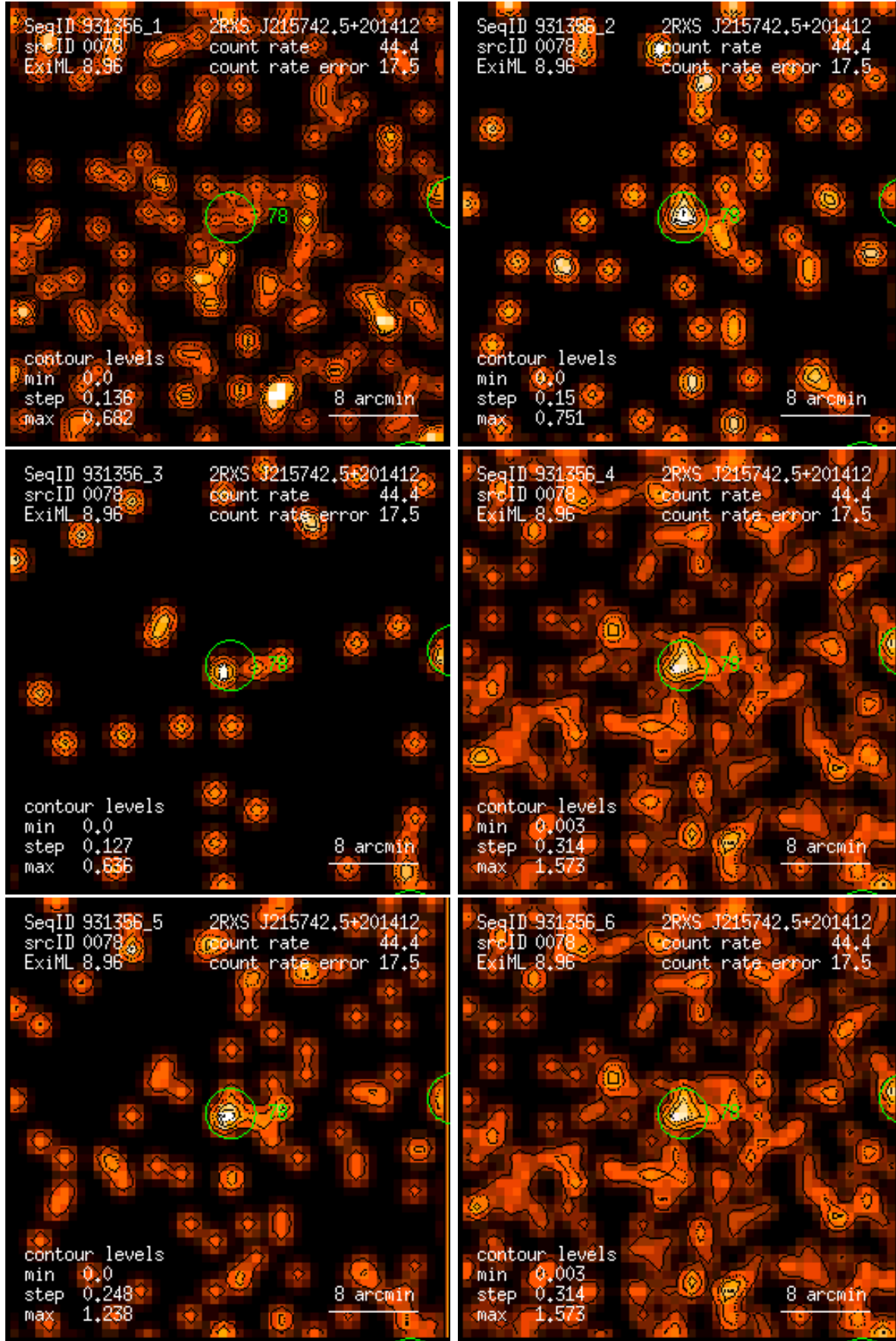
Figure 78: RASS 931356: detection 0078: band rate images, Gaussian filter: (1) PSPC channels 11 – 41, (2) 52 – 90, (3) 91 – 201, (4) 11 – 235, (5) 52 – 201, (6) 11 – 201. Broad band rates in counts/ks. Band rate contour levels in counts/ks/arcmin 2 .
