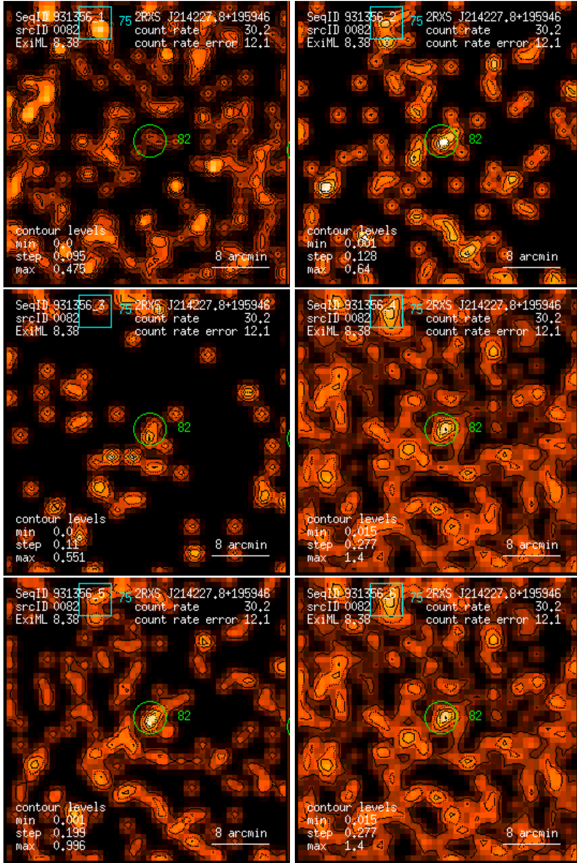
Figure 82: RASS 931356: detection 0082: band rate images, Gaussian filter: (1) PSPC channels 11 – 41, (2) 52 – 90, (3) 91 – 201, (4) 11 – 235, (5) 52 – 201, (6) 11 – 201. Broad band rates in counts/ks. Band rate contour levels in counts/ks/arcmin 2 .
