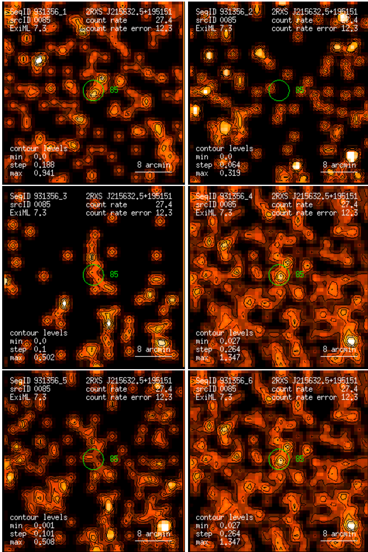
Figure 85: RASS 931356: detection 0085: band rate images, Gaussian filter: (1) PSPC channels 11 – 41, (2) 52 – 90, (3) 91 – 201, (4) 11 – 235, (5) 52 – 201, (6) 11 – 201. Broad band rates in counts/ks. Band rate contour levels in counts/ks/arcmin 2 .
