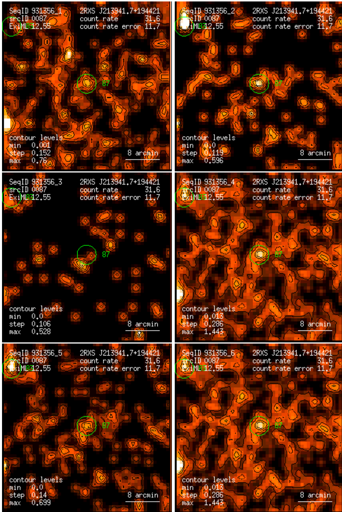
Figure 87: RASS 931356: detection 0087: band rate images, Gaussian filter: (1) PSPC channels 11 – 41, (2) 52 – 90, (3) 91 – 201, (4) 11 – 235, (5) 52 – 201, (6) 11 – 201. Broad band rates in counts/ks. Band rate contour levels in counts/ks/arcmin 2 .
