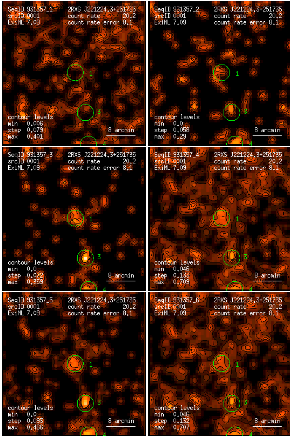
Figure 1: RASS 931357: detection 0001: band rate images, Gaussian filter: (1) PSPC channels 11 – 41, (2) 52 – 90, (3) 91 – 201, (4) 11 – 235, (5) 52 – 201, (6) 11 – 201. Broad band rates in counts/ks. Band rate contour levels in counts/ks/arcmin 2 .
