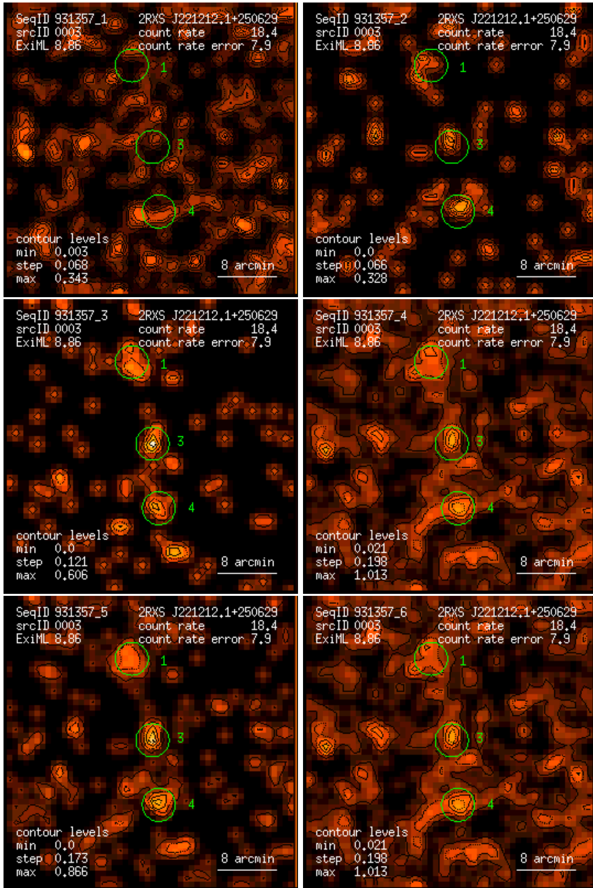
Figure 3: RASS 931357: detection 0003: band rate images, Gaussian filter: (1) PSPC channels 11 – 41, (2) 52 – 90, (3) 91 – 201, (4) 11 – 235, (5) 52 – 201, (6) 11 – 201. Broad band rates in counts/ks. Band rate contour levels in counts/ks/arcmin 2 .
