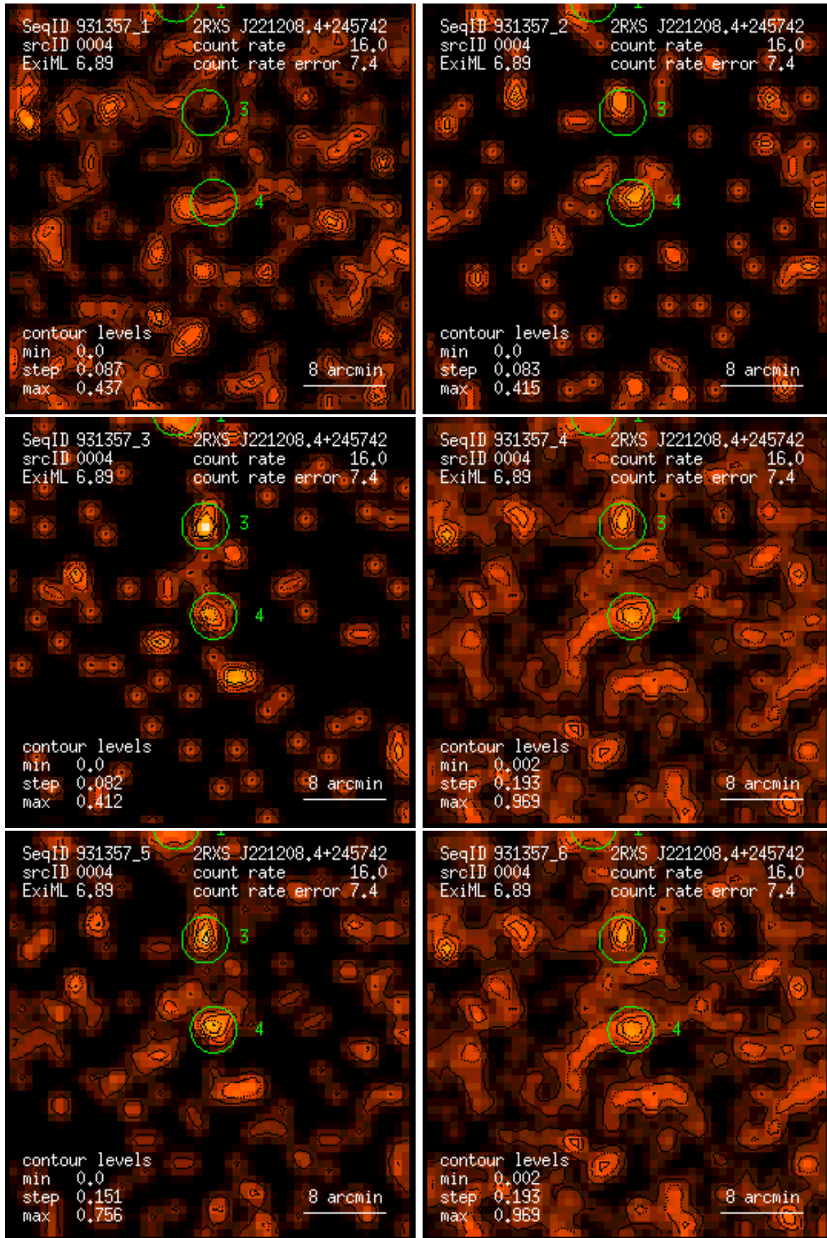
Figure 4: RASS 931357: detection 0004: band rate images, Gaussian filter: (1) PSPC channels 11 – 41, (2) 52 – 90, (3) 91 – 201, (4) 11 – 235, (5) 52 – 201, (6) 11 – 201. Broad band rates in counts/ks. Band rate contour levels in counts/ks/arcmin 2 .
