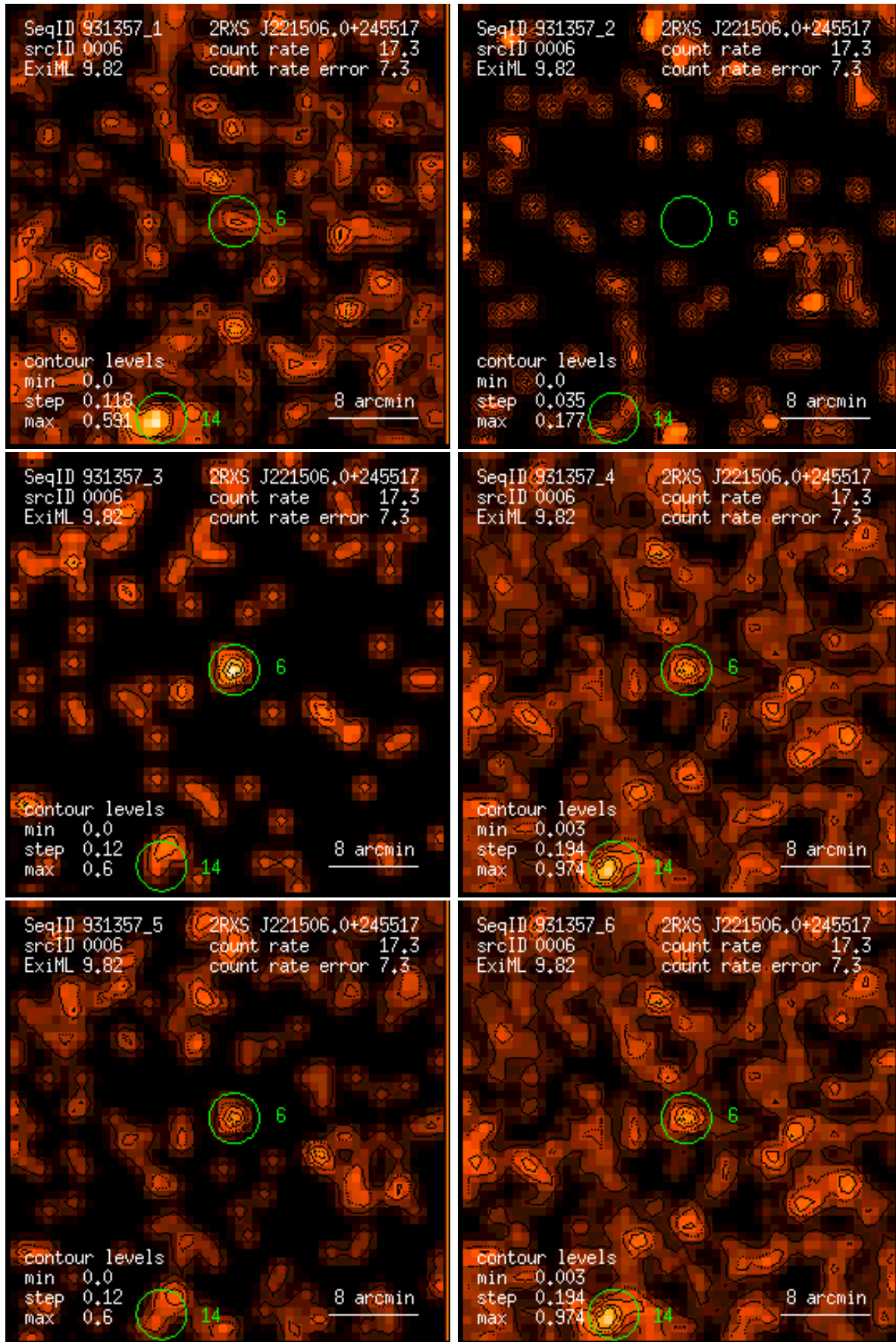
Figure 6: RASS 931357: detection 0006: band rate images, Gaussian filter: (1) PSPC channels 11 – 41, (2) 52 – 90, (3) 91 – 201, (4) 11 – 235, (5) 52 – 201, (6) 11 – 201. Broad band rates in counts/ks. Band rate contour levels in counts/ks/arcmin 2 .
