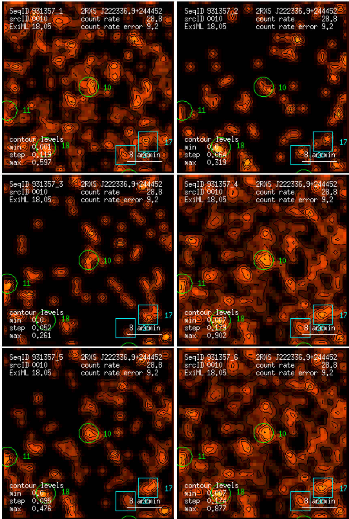
Figure 10: RASS 931357: detection 0010: band rate images, Gaussian filter: (1) PSPC channels 11 – 41, (2) 52 – 90, (3) 91 – 201, (4) 11 – 235, (5) 52 – 201, (6) 11 – 201. Broad band rates in counts/ks. Band rate contour levels in counts/ks/arcmin 2 .
