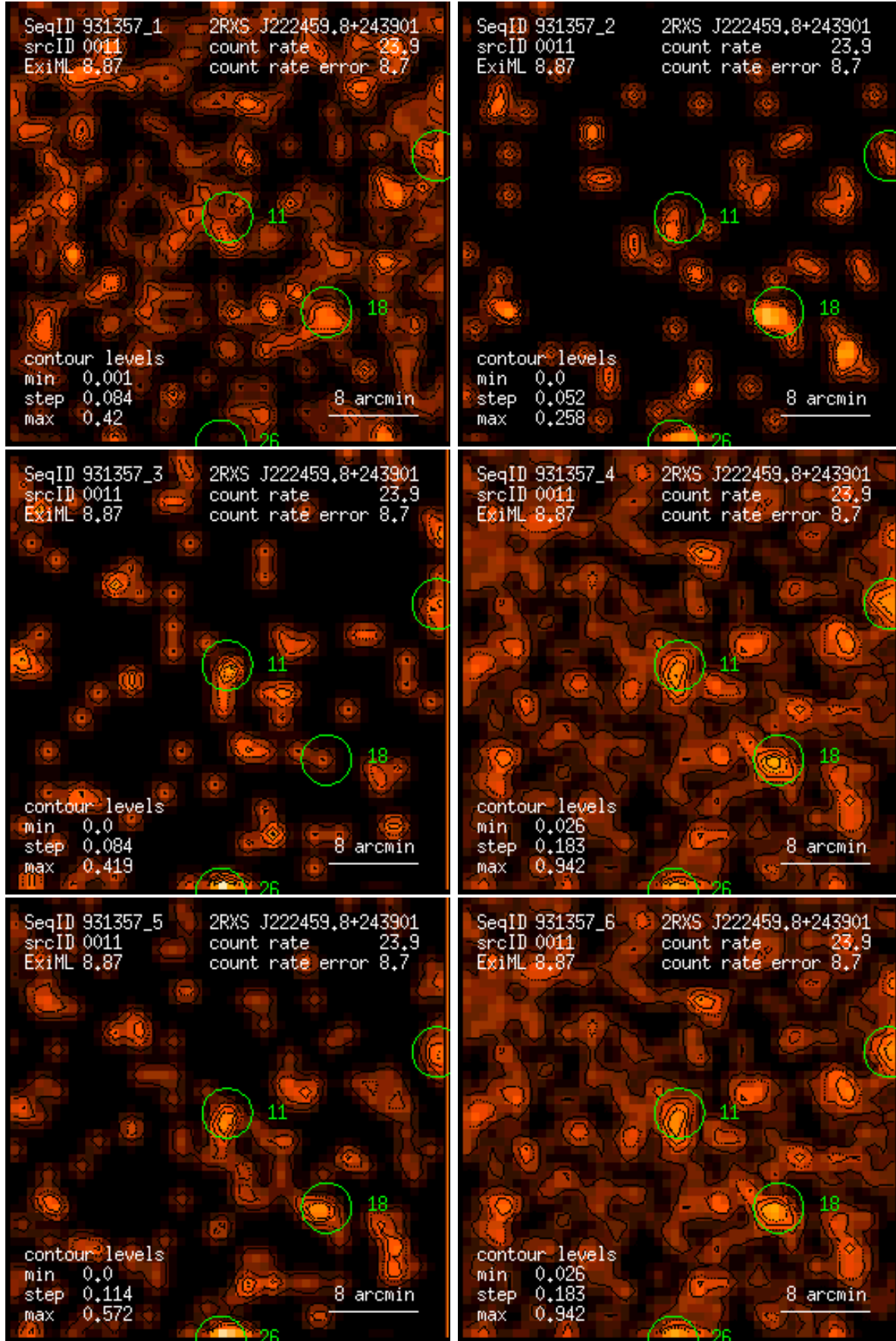
Figure 11: RASS 931357: detection 0011: band rate images, Gaussian filter: (1) PSPC channels 11 – 41, (2) 52 – 90, (3) 91 – 201, (4) 11 – 235, (5) 52 – 201, (6) 11 – 201. Broad band rates in counts/ks. Band rate contour levels in counts/ks/arcmin 2 .
